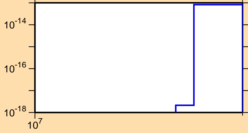
\sigma vs. E for ^{170}\text{Ho}(n,\text{He3})
