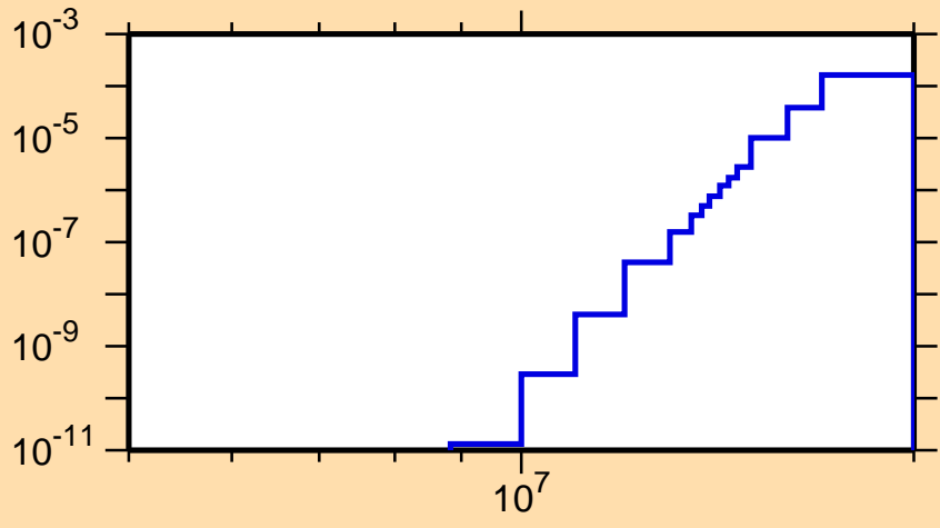
\sigma vs. E for ^{170}\text{Ho}(n,n\alpha)
