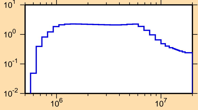
\sigma vs. E for ^{170}\text{Ho}(n,n\text{cont.})
