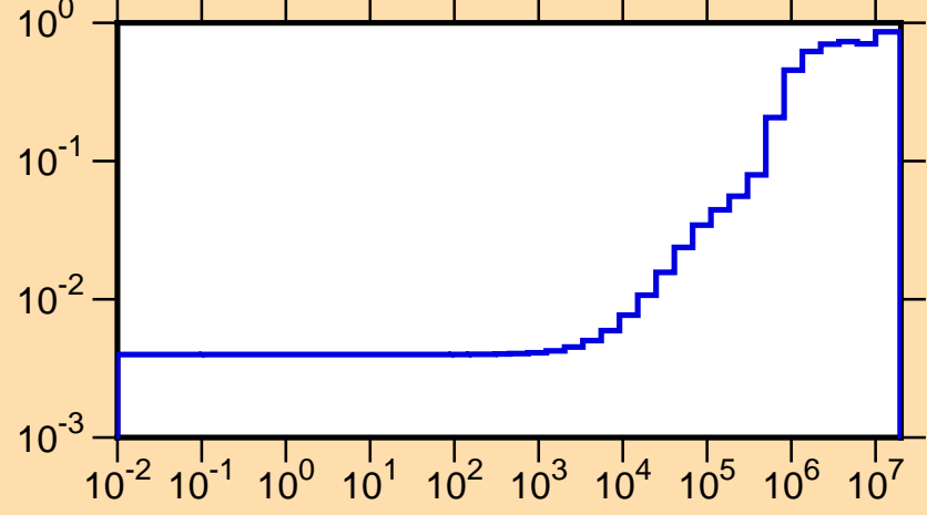
\mu vs. E for ^{170}\text{Ho}(\text{mt251})
