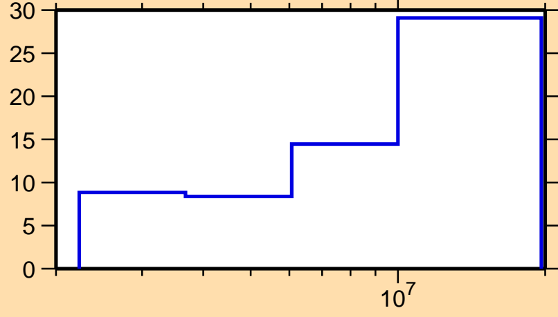
\Delta\sigma/\sigma vs. E for ^{170}\text{Ho}(n,n\text{cont.})
