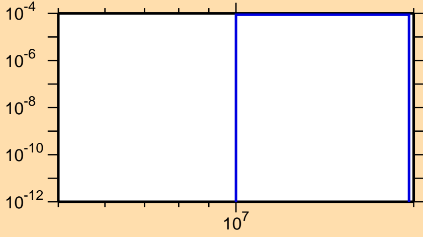
\sigma vs. E for ^{170}\text{Ho}(n,np)
