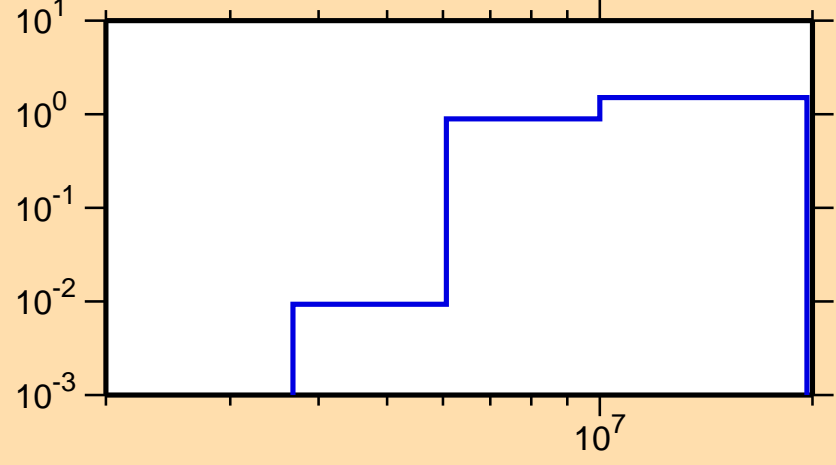
\sigma vs. E for ^{170}\text{Ho}(n,2n)
