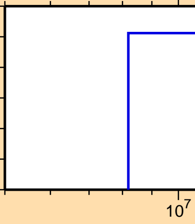
\sigma vs. E for ^{170}\text{Ho}(n,t)
