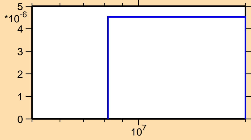
\sigma vs. E for ^{170}\text{Ho}(n,\alpha)
