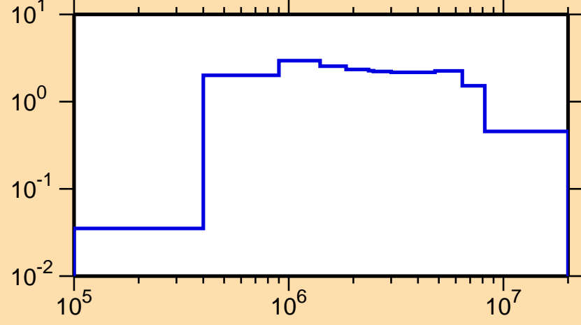
\sigma vs. E for ^{170}\text{Ho}(n,\text{inel.})
