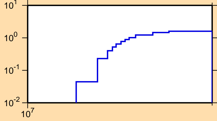
\sigma vs. E for ^{170}\text{Ho}(n,3n)
