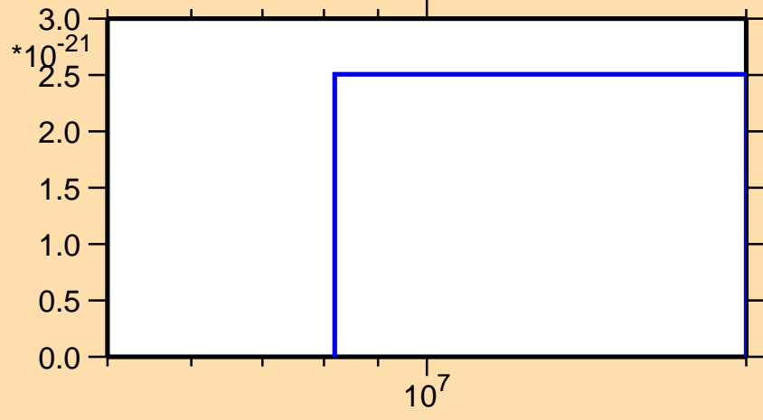
\sigma vs. E for ^{170}\text{Ho} (mt 42)
