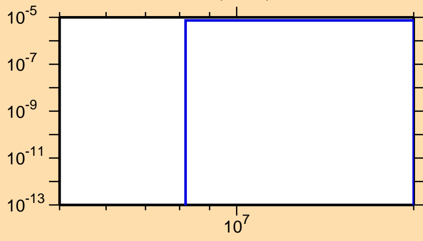
\sigma vs. E for ^{170}\text{Ho}(n,\alpha)
