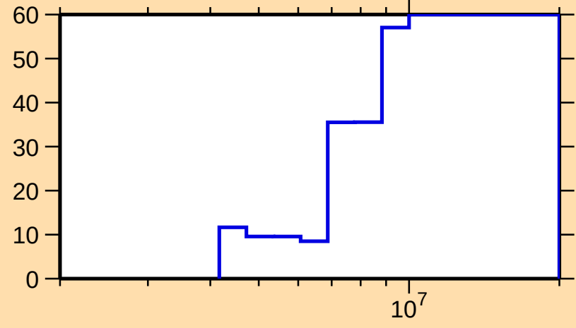
\Delta\sigma/\sigma vs. E for ^{171}\text{Ho}(n,n\text{cont.})
