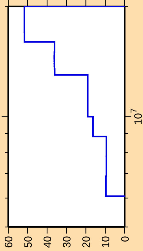
\Delta\sigma/\sigma vs. E for ^{171}\text{Ho}(n,2n)
