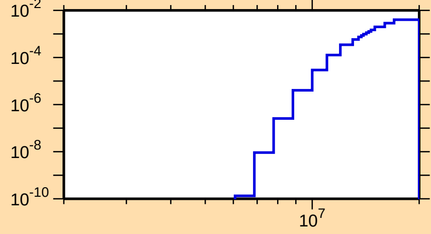
\sigma vs. E for ^{171}\text{Ho}(n,p)
