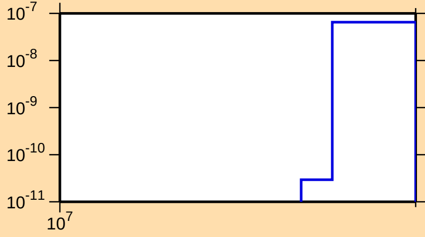
\sigma vs. E for ^{171}\text{Ho}(n,2np)
