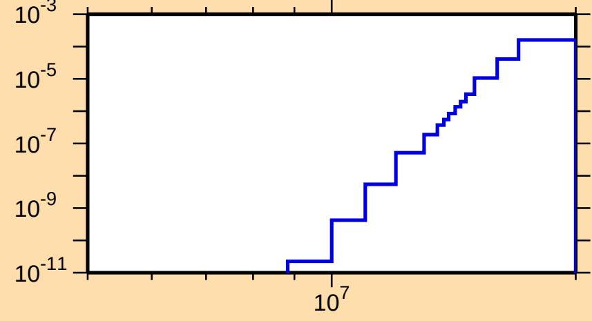
\sigma vs. E for ^{171}\text{Ho}(n,\alpha)
