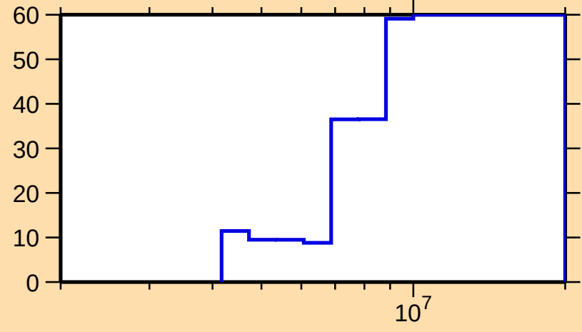
\Delta\sigma/\sigma vs. E for ^{171}\text{Ho}(n,\text{inel.})
