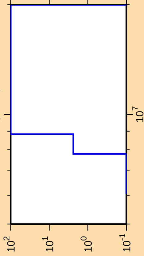
\Delta\sigma/\sigma vs. E for ^{171}\text{Ho}(n,\alpha)
