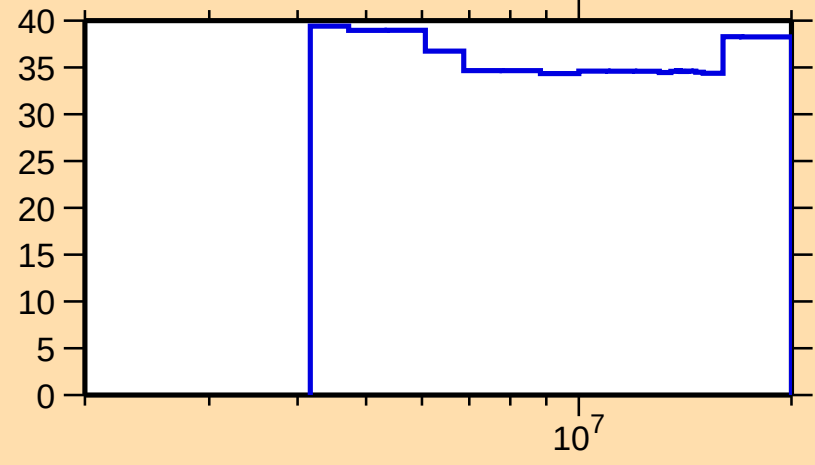
\Delta\sigma/\sigma vs. E for ^{171}\text{Ho}(n,\text{el.})
