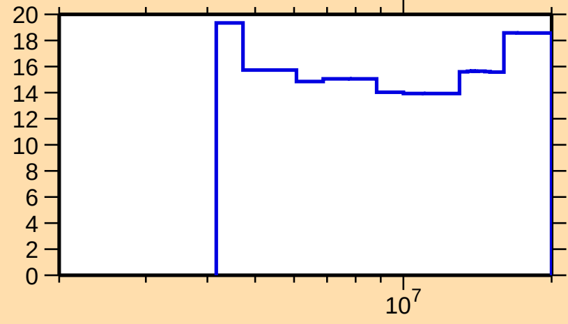
\Delta\sigma/\sigma vs. E for ^{171}\text{Ho}(n,\text{tot.})
