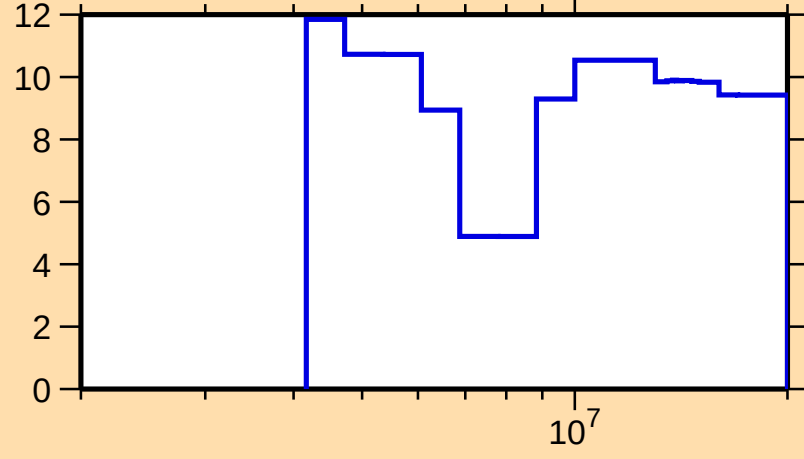
\Delta\sigma/\sigma vs. E for ^{171}\text{Ho}(n,\text{nonel.})
