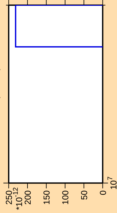
\Delta\sigma/\sigma vs. E for ^{171}\text{Ho} (mt 42)
