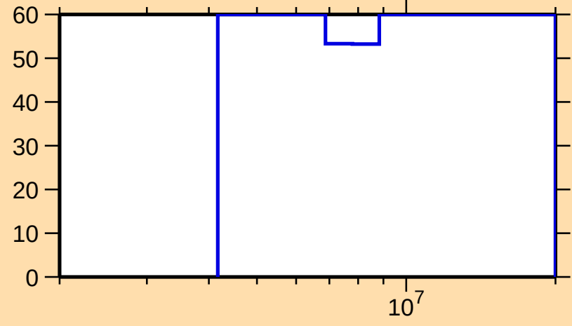
\Delta\sigma/\sigma vs. E for ^{171}\text{Ho}(n,\gamma)
