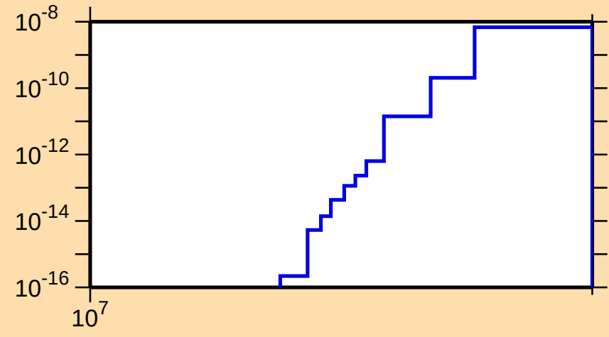
\sigma vs. E for ^{171}\text{Ho}(n,2n\alpha)
