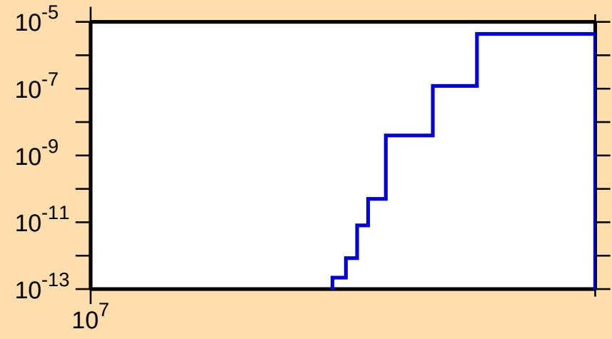
\sigma vs. E for ^{171}\text{Ho}(n,nt)
