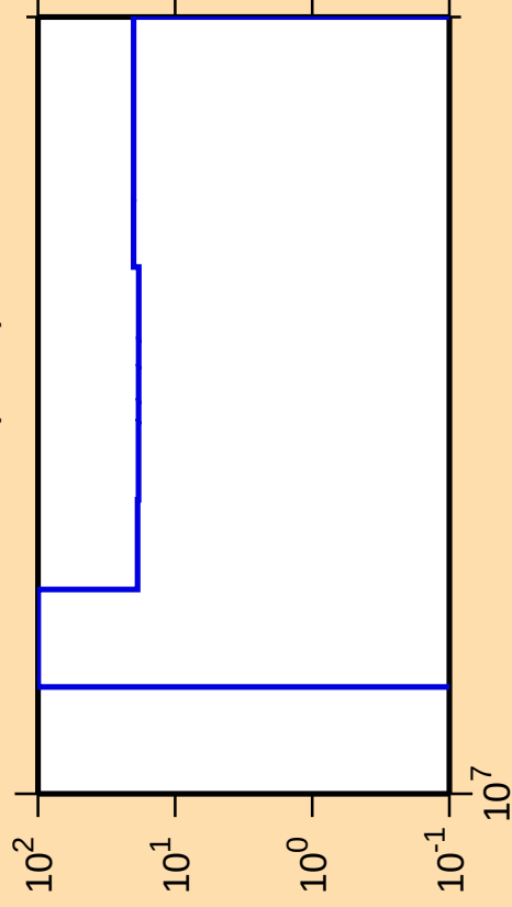
\Delta\sigma/\sigma vs. E for ^{171}\text{Ho}(n,3n)
