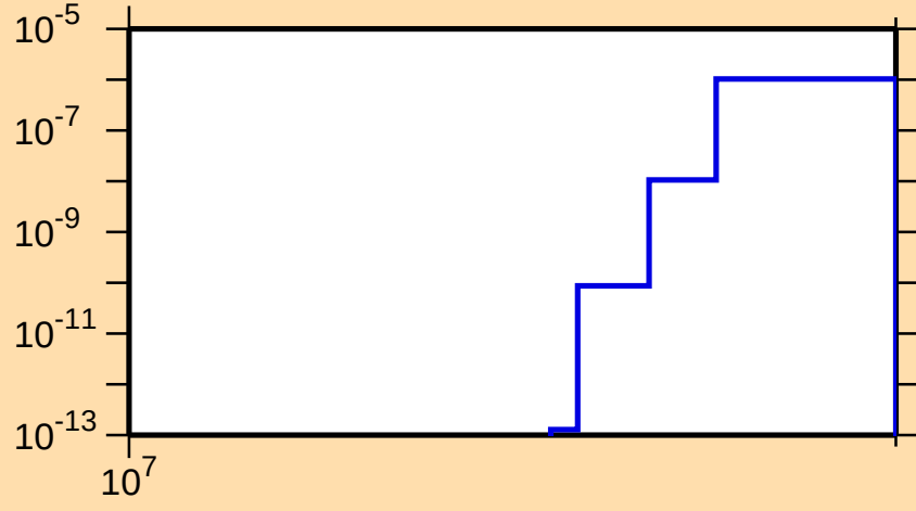
\sigma vs. E for ^{171}\text{Ho}(n,\text{nd})
