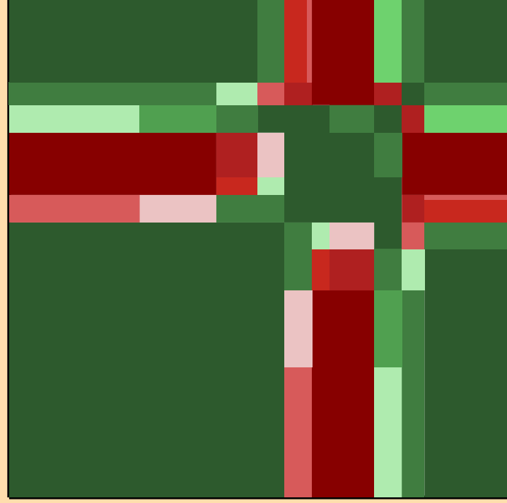
\sigma vs. E for ^{171}\text{Ho}(n,\text{inel.})
