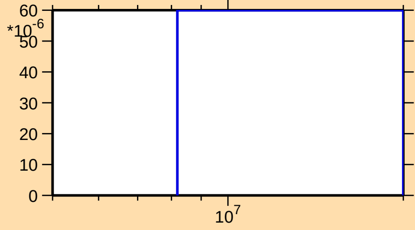
\sigma vs. E for ^{171}\text{Ho}(n,d)
