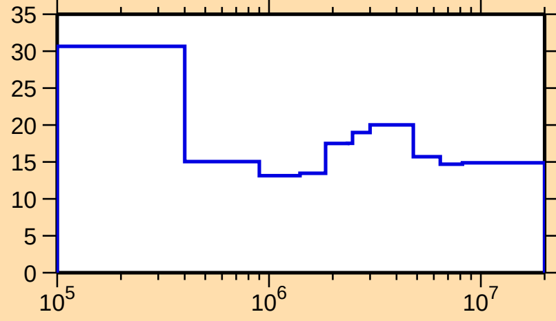
\Delta\sigma/\sigma vs. E for ^{171}\text{Ho}(\text{n,tot.})
