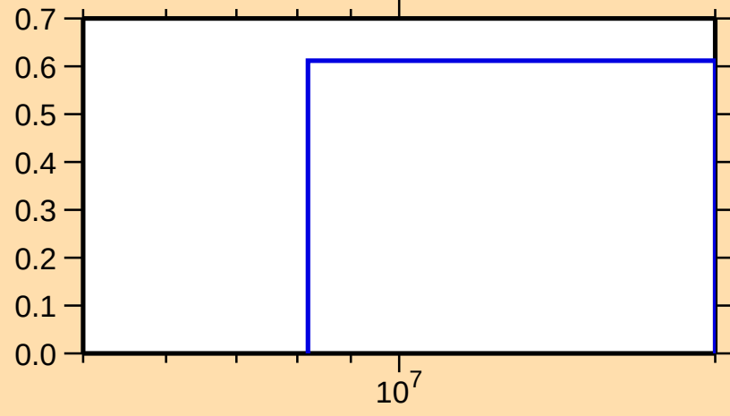
\sigma vs. E for ^{171}\text{Ho}(n,3n)
