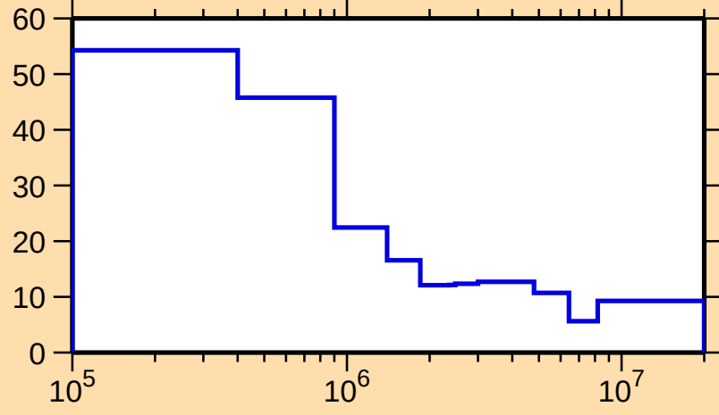
\Delta\sigma/\sigma vs. E for ^{171}\text{Ho}(n,n\text{onel.})
