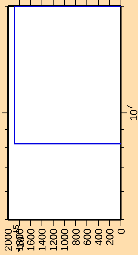
\Delta\sigma/\sigma vs. E for ^{171}\text{Ho}(\text{mt } 42)
