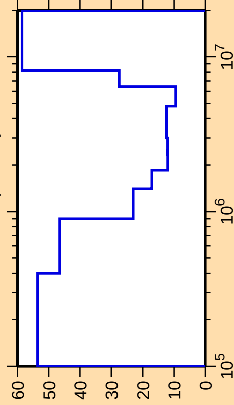
\Delta\sigma/\sigma vs. E for ^{171}\text{Ho}(n,\text{inel.})
