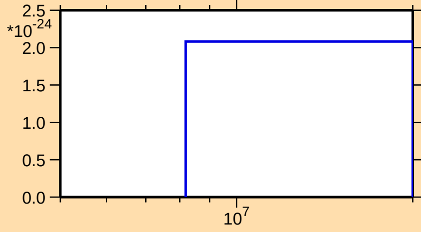
\sigma vs. E for ^{171}\text{Ho}(\text{mt } 42)
