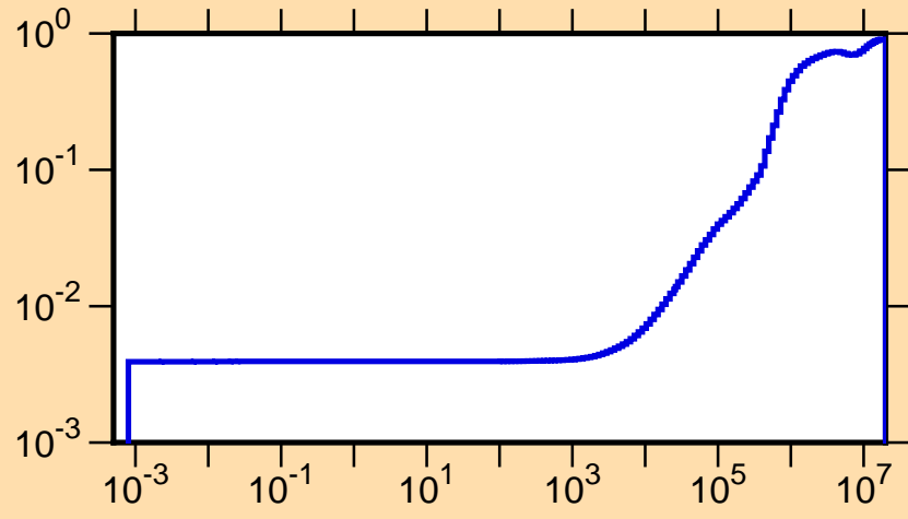
\mu vs. E for ^{172}\text{Ho}(\text{mt251})
