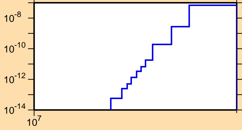
\sigma vs. E for ^{172}\text{Ho}(n,2n\alpha)
