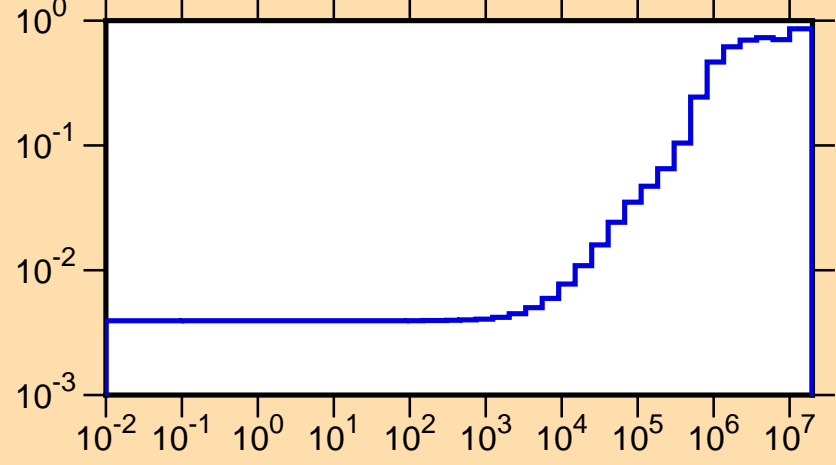
\mu vs. E for ^{172}\text{Ho}(\text{mt251})
