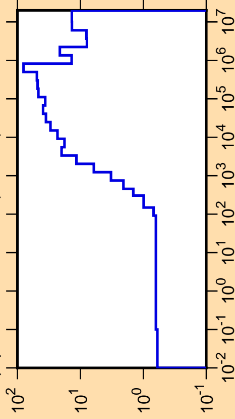
\Delta\mu/\mu vs. E for ^{172}\text{Ho}(\text{mt251})
