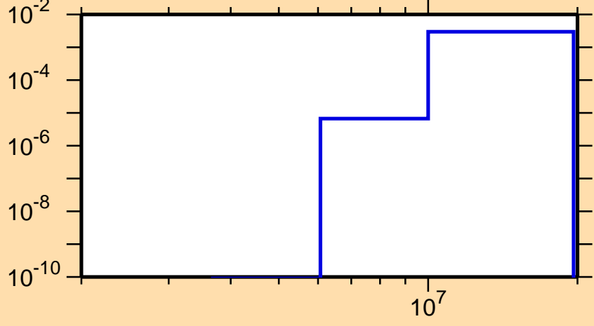
\sigma vs. E for ^{172}\text{Ho}(n,p)
