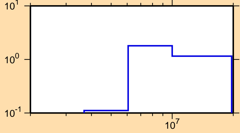
\sigma vs. E for ^{172}\text{Ho}(n,2n)
