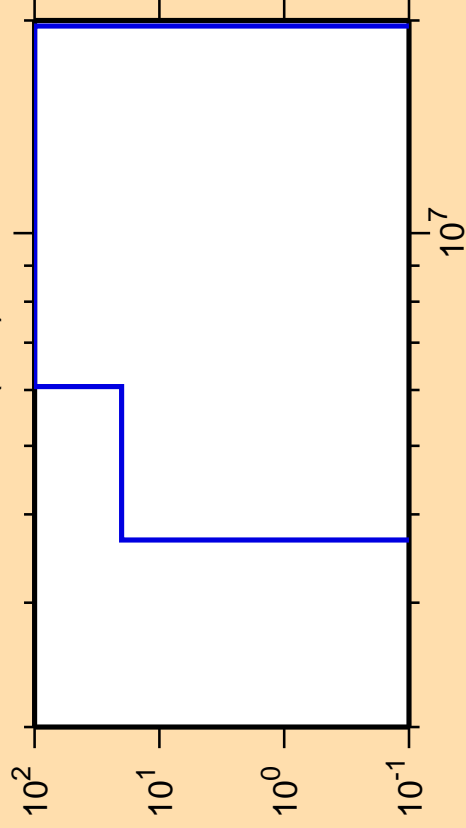
\Delta\sigma/\sigma vs. E for ^{172}\text{Ho}(n,\alpha)
