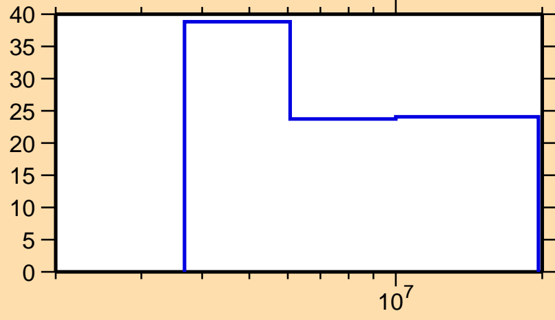
\Delta\sigma/\sigma vs. E for ^{172}\text{Ho}(n,2n)
