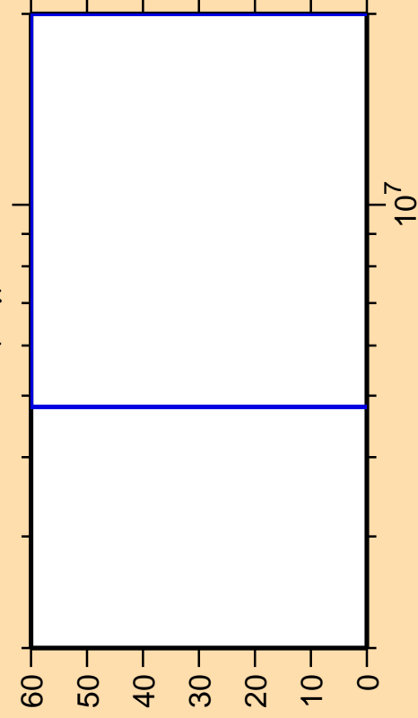
\Delta\sigma/\sigma vs. E for ^{172}\text{Ho}(n,\gamma)
