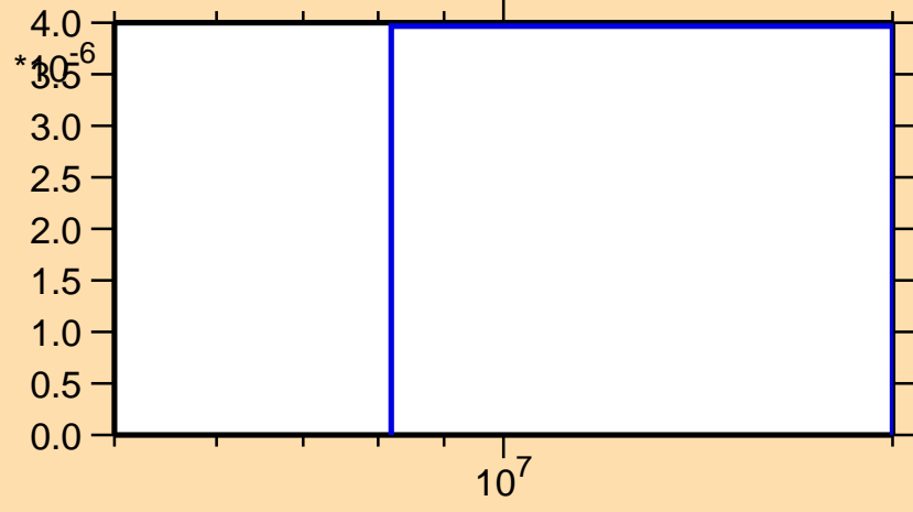
\sigma vs. E for ^{172}\text{Ho}(n,\alpha)
