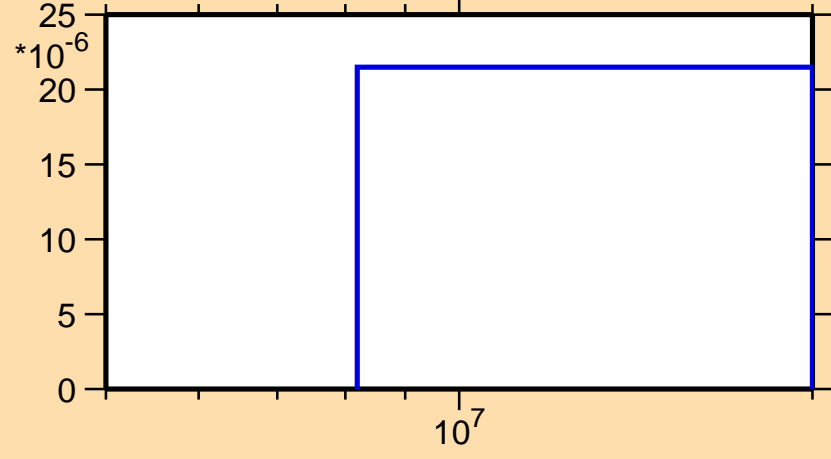
\sigma vs. E for ^{172}\text{Ho}(n,t)
