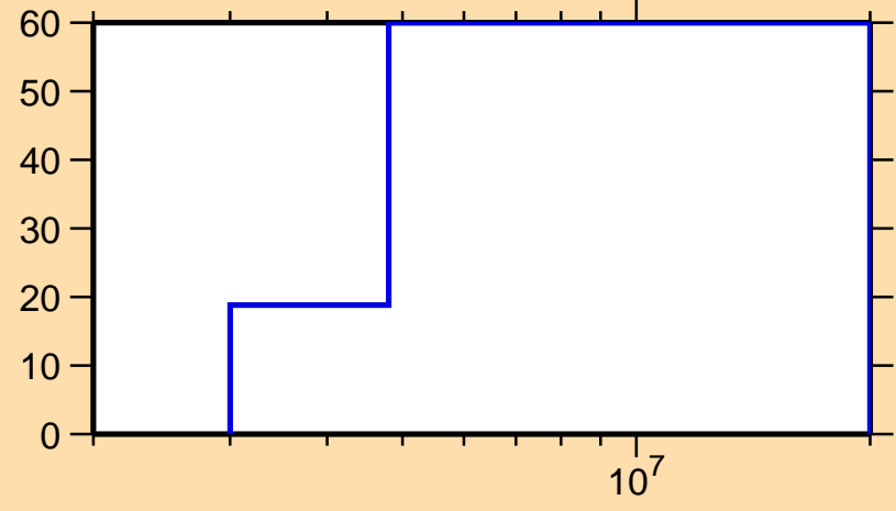
\Delta\sigma/\sigma vs. E for ^{172}\text{Ho}(n,ncont.)
