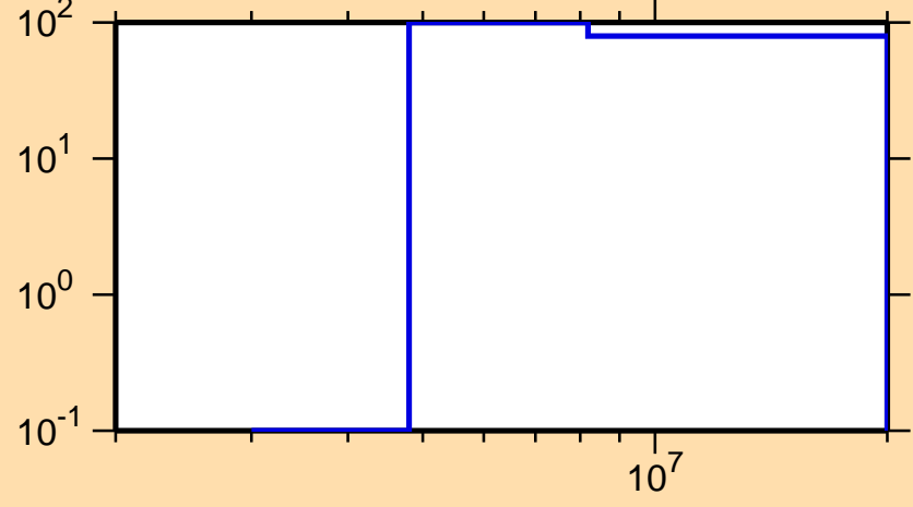
\Delta\sigma/\sigma vs. E for ^{172}\text{Ho}(n,p)
