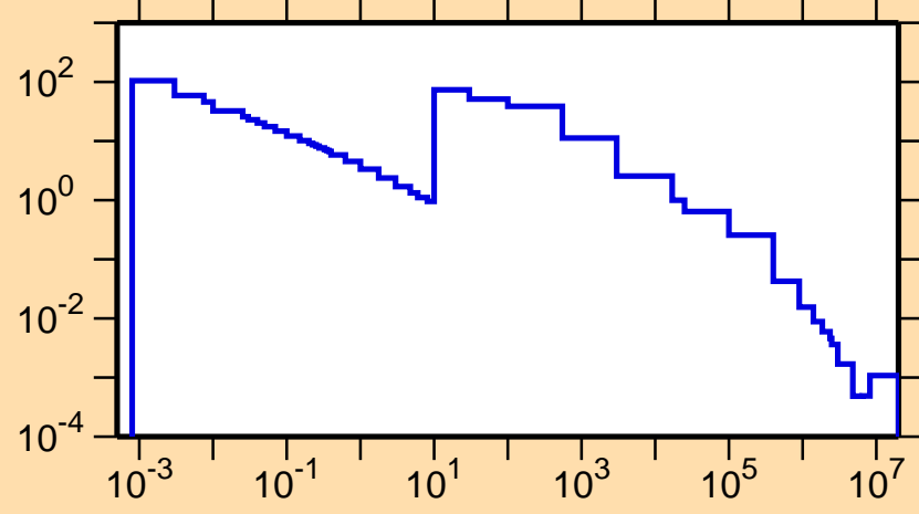
\sigma vs. E for ^{172}\text{Ho}(n,\gamma)
