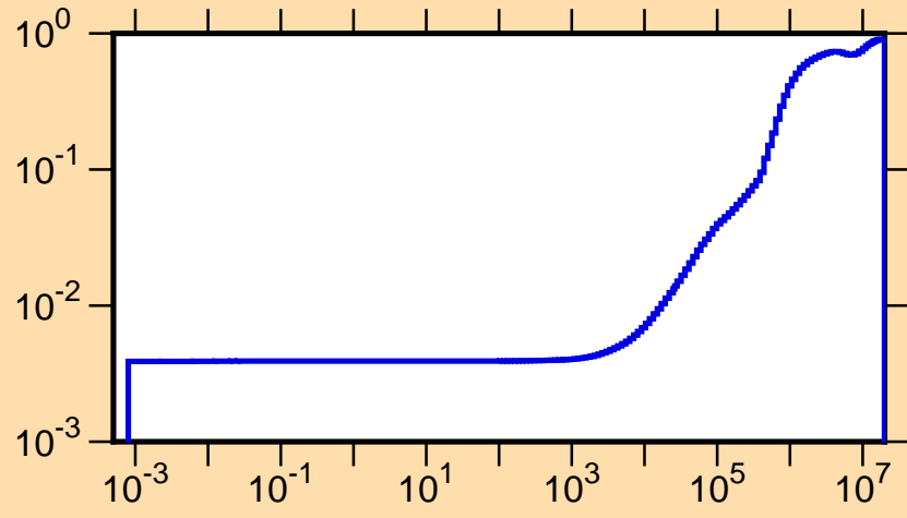
\mu vs. E for ^{173}\text{Ho}(\text{mt251})
