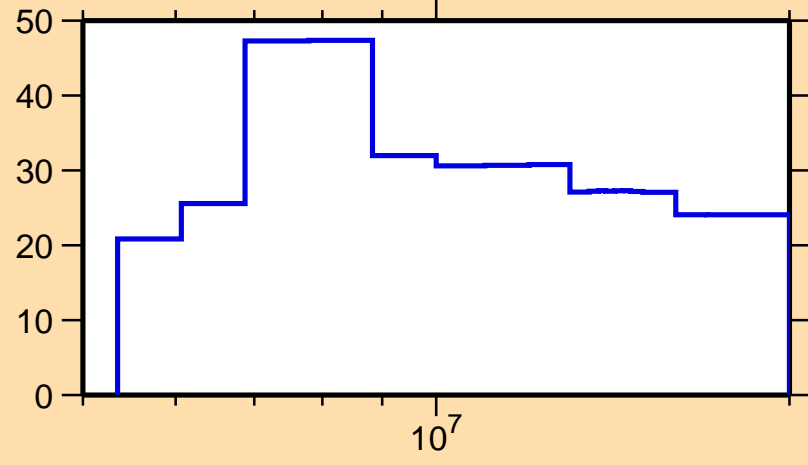
\Delta\sigma/\sigma vs. E for ^{173}\text{Ho}(n,\text{inel.})
