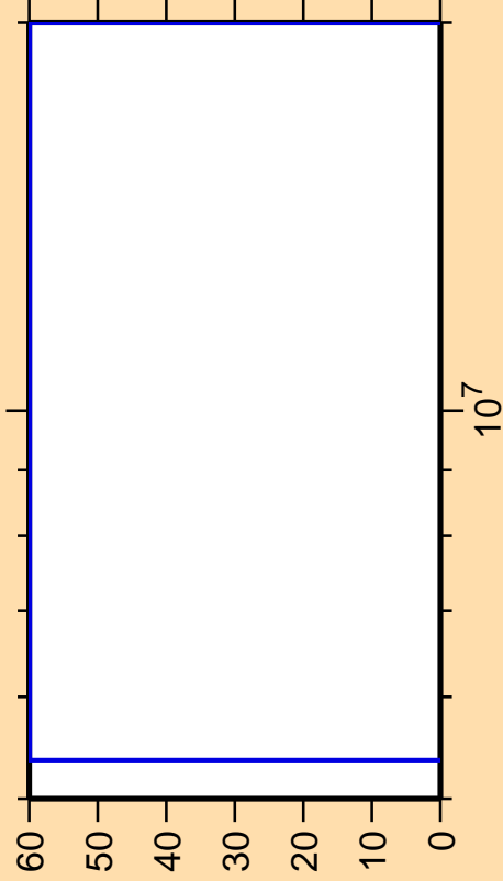
\Delta\sigma/\sigma vs. E for ^{173}\text{Ho}(n,\gamma)
