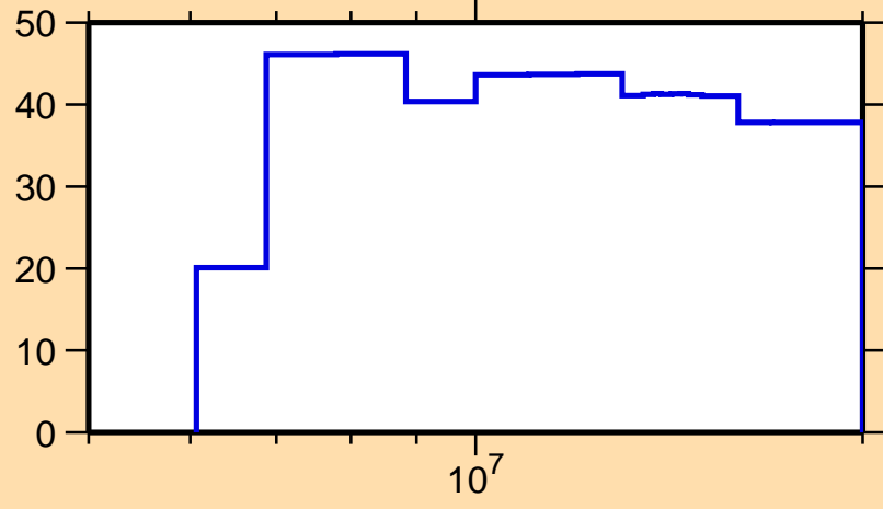
\Delta\sigma/\sigma vs. E for ^{173}\text{Ho}(n,ncont.)
