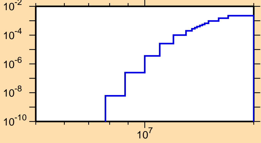
\sigma vs. E for ^{173}\text{Ho}(n,p)
