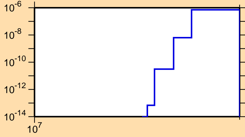
\sigma vs. E for ^{173}\text{Ho}(n,\text{nd})
