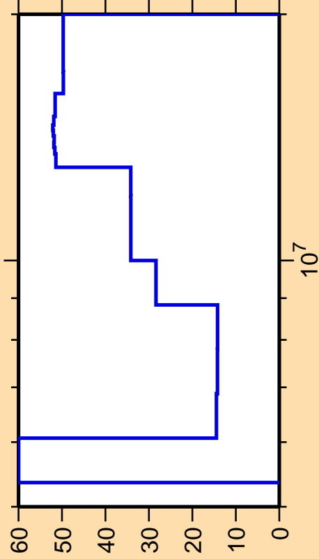
\Delta\sigma/\sigma vs. E for ^{173}\text{Ho}(n,2n)
