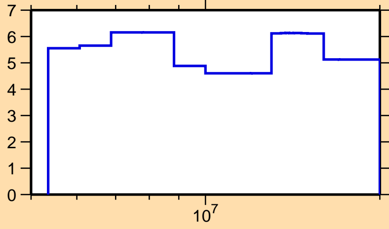
\Delta\sigma/\sigma vs. E for ^{173}\text{Ho}(n,\text{nonel.})
