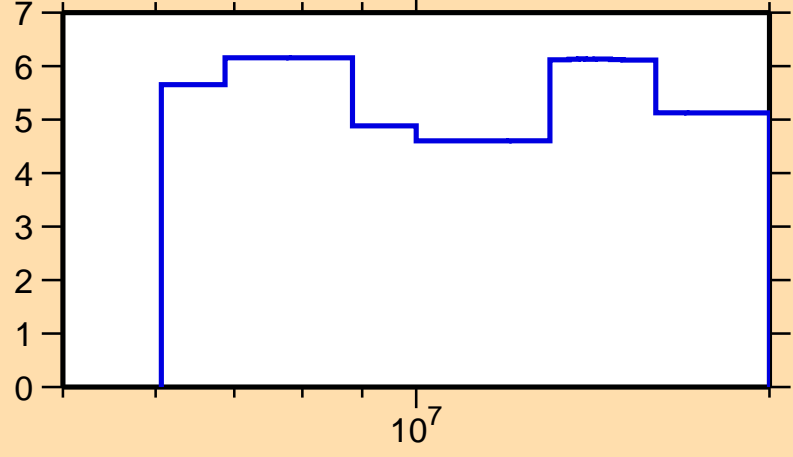
\Delta\sigma/\sigma vs. E for ^{173}\text{Ho}(n,\text{nonel.})
