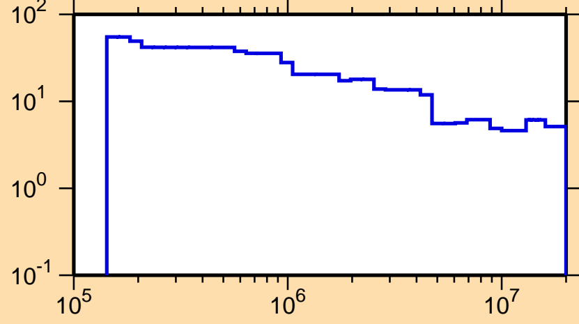
\Delta\sigma/\sigma vs. E for ^{173}\text{Ho}(n,n\text{onel.})
