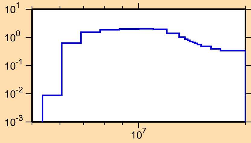
\sigma vs. E for ^{173}\text{Ho}(n,2n)
