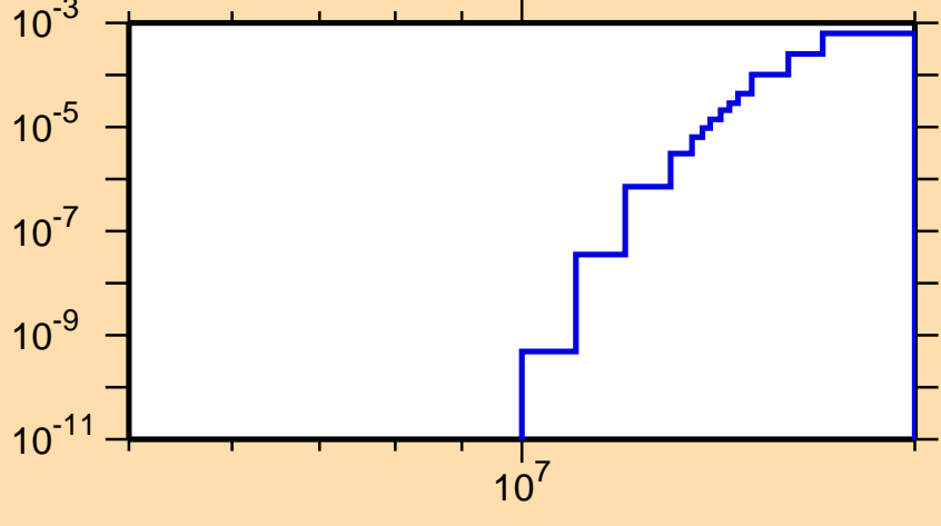
\sigma vs. E for ^{173}\text{Ho}(n,d)
