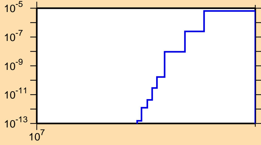
\sigma vs. E for ^{173}\text{Ho}(n,nt)
