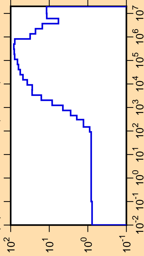
\Delta\mu/\mu vs. E for ^{173}\text{Ho}(\text{mt251})
