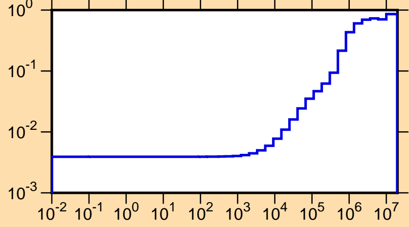
\mu vs. E for ^{173}\text{Ho}(\text{mt251})
