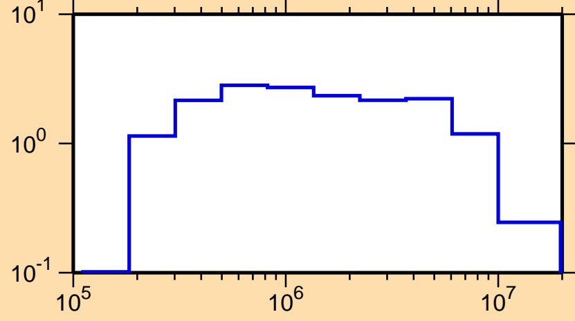
\sigma vs. E for ^{173}\text{Ho}(n,\text{inel.})
