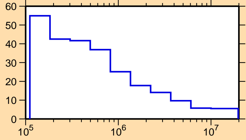
\Delta\sigma/\sigma vs. E for ^{173}\text{Ho}(n,n\text{onel.})
