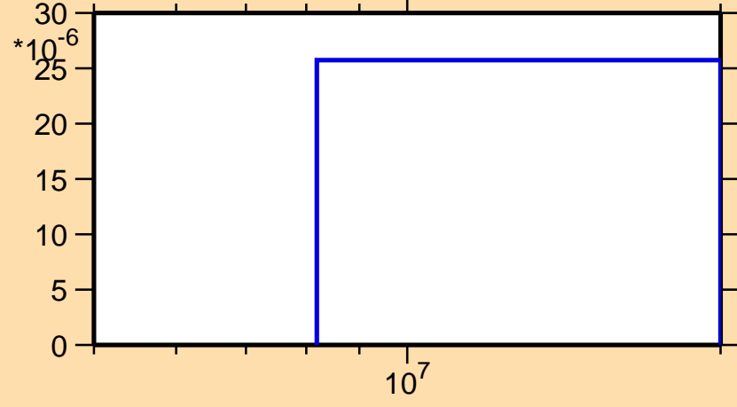
\sigma vs. E for ^{173}\text{Ho}(n,np)
