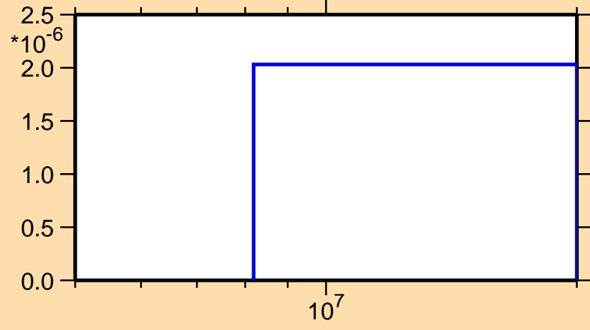
\sigma vs. E for ^{173}\text{Ho}(n,\alpha)
