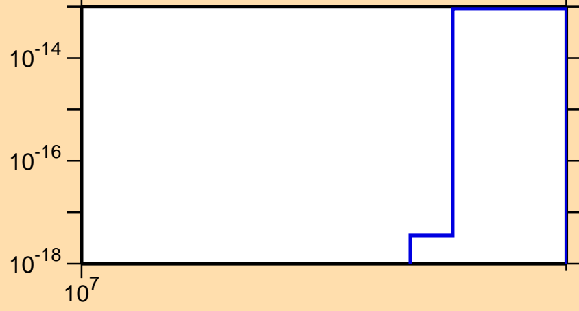
\sigma vs. E for ^{174}\text{Ho} (mt 11)
