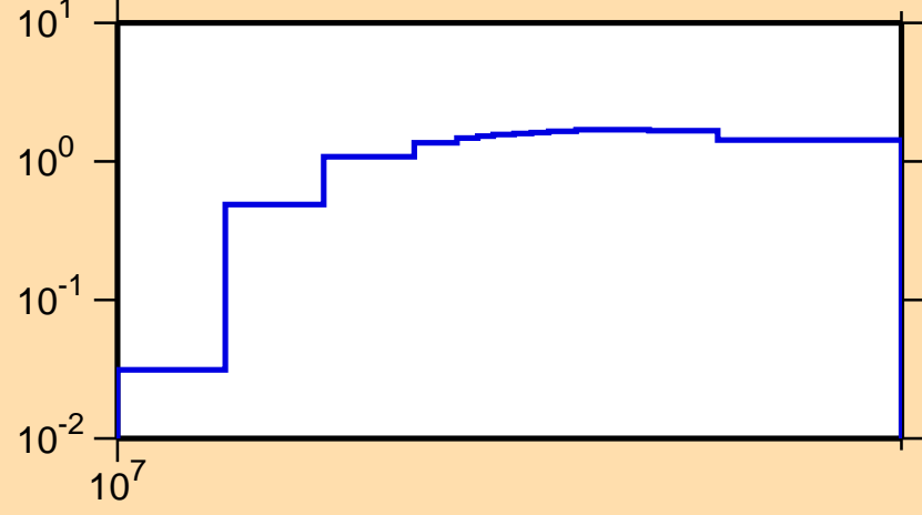
\sigma vs. E for ^{174}\text{Ho}(n,3n)
