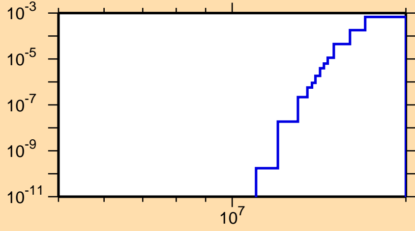
\sigma vs. E for ^{174}\text{Ho}(n,np)
