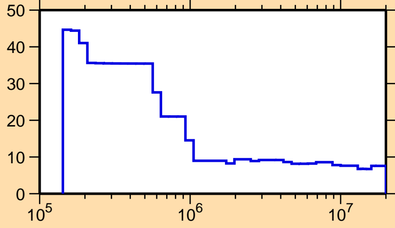
\Delta\sigma/\sigma vs. E for ^{174}\text{Ho}(n,n\text{onel.})
