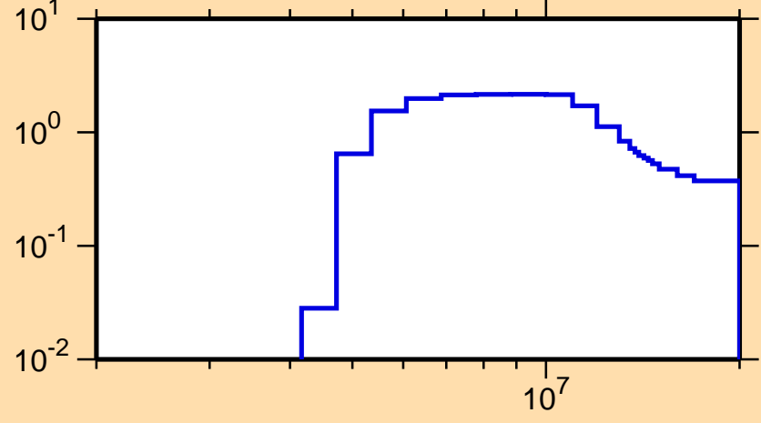
\sigma vs. E for ^{174}\text{Ho}(n,2n)
