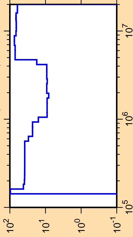
\Delta\sigma/\sigma vs. E for ^{174}\text{Ho}(n,\text{ncont.})
