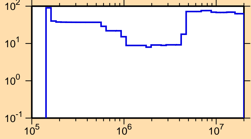
\Delta\sigma/\sigma vs. E for ^{174}\text{Ho}(n,\text{inel.})
