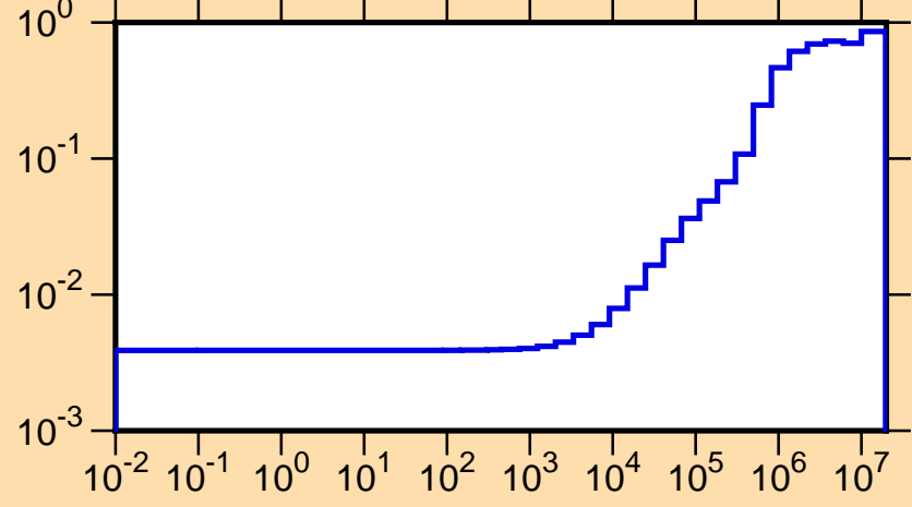
\mu vs. E for ^{174}\text{Ho}(\text{mt251})
