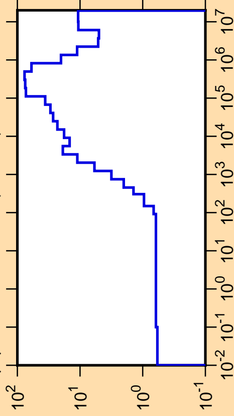
\Delta\mu/\mu vs. E for ^{174}\text{Ho}(\text{mt251})
