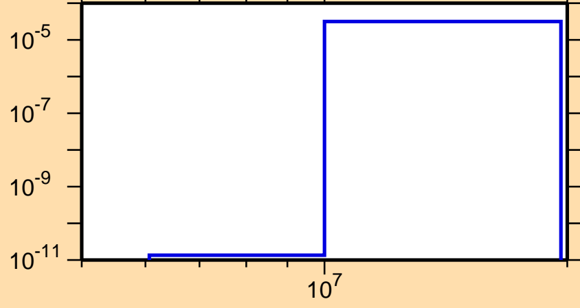
\sigma vs. E for ^{174}\text{Ho}(n,t)
