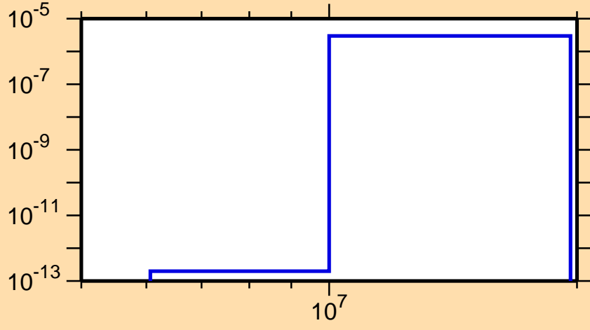
\sigma vs. E for ^{174}\text{Ho}(n,n\alpha)
