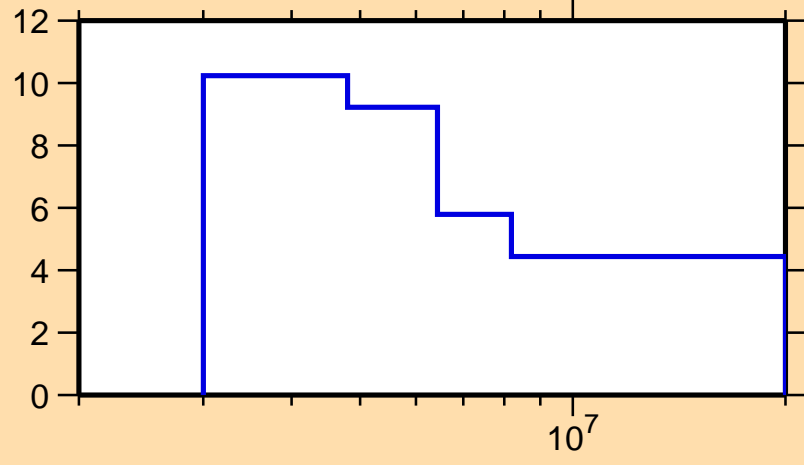
\Delta\sigma/\sigma vs. E for ^{174}\text{Ho}(n,\text{tot.})
