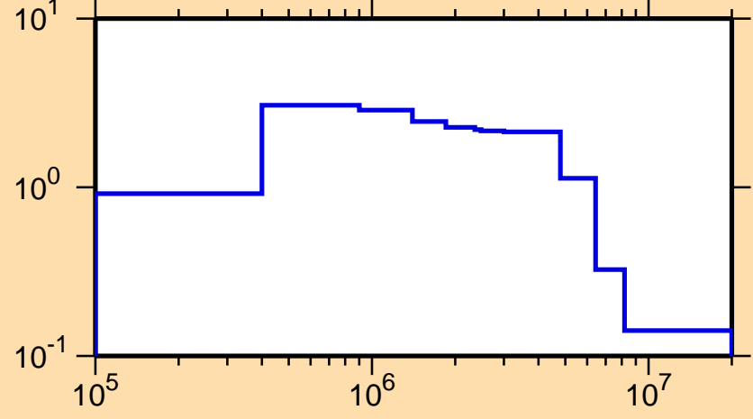
\sigma vs. E for ^{174}\text{Ho}(n,n\text{cont.})
