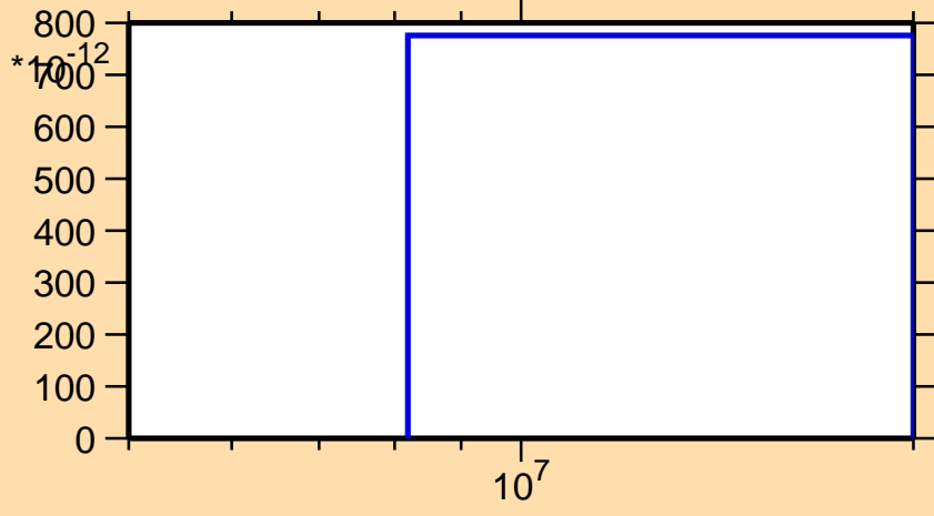
\sigma vs. E for ^{174}\text{Ho}(n,2n\alpha)
