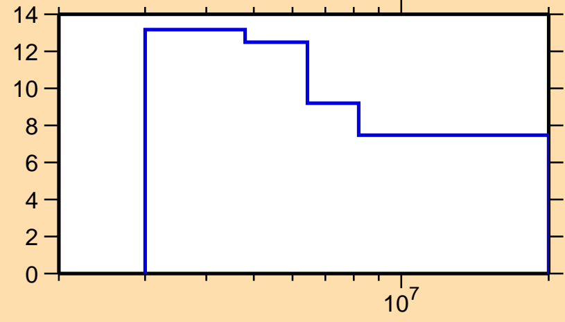
\Delta\sigma/\sigma vs. E for ^{174}\text{Ho}(n,\text{el.})
