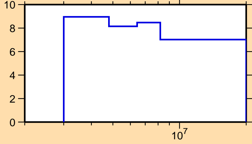
\Delta\sigma/\sigma vs. E for ^{174}\text{Ho}(n,\text{nonel.})
