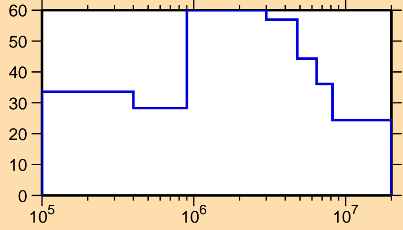
\Delta\sigma/\sigma vs. E for ^{174}\text{Ho}(n,n_1)
