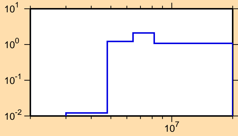
\sigma vs. E for ^{174}\text{Ho}(n,2n)
