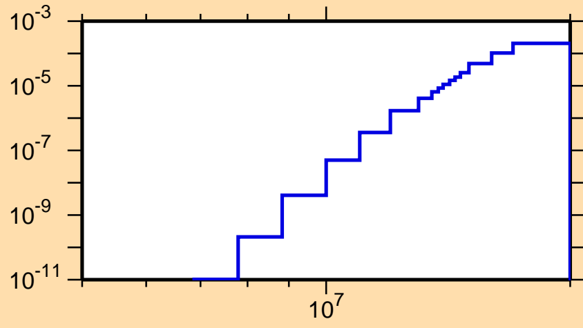
\sigma vs. E for ^{175}\text{Ho}(n,\alpha)
