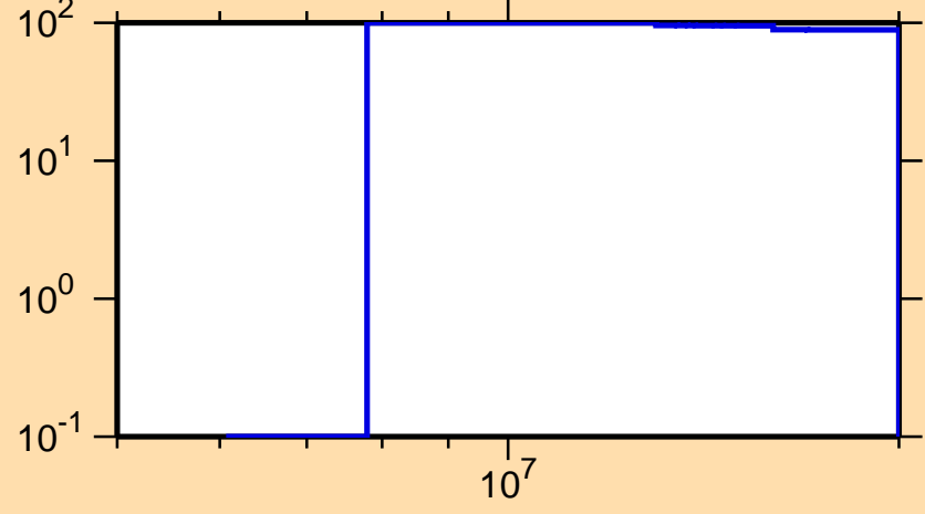
\Delta\sigma/\sigma vs. E for ^{175}\text{Ho}(n,p)
