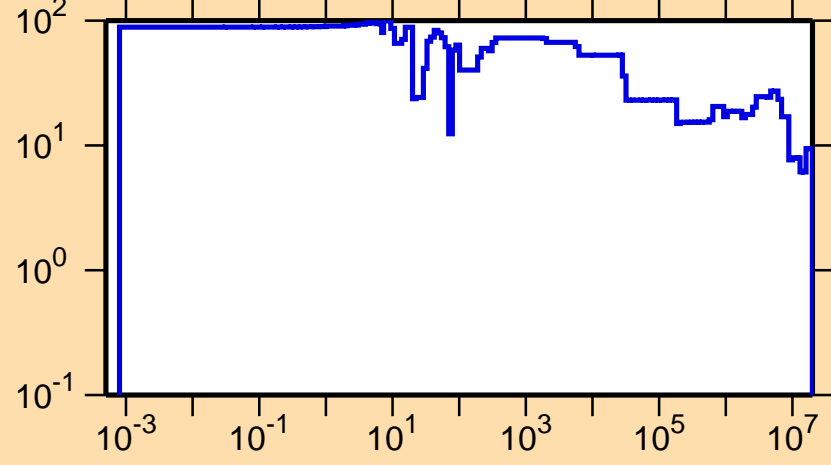
\Delta\sigma/\sigma vs. E for ^{175}\text{Ho}(n,\text{el.})
