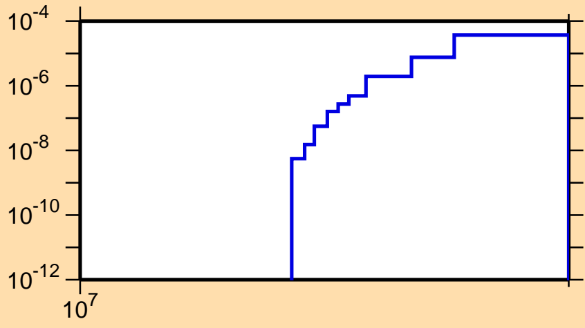
\sigma vs. E for ^{119}\text{La}(n,2np)
