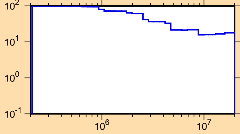
\Delta\sigma/\sigma vs. E for ^{119}\text{La}(n,\text{inel.})
