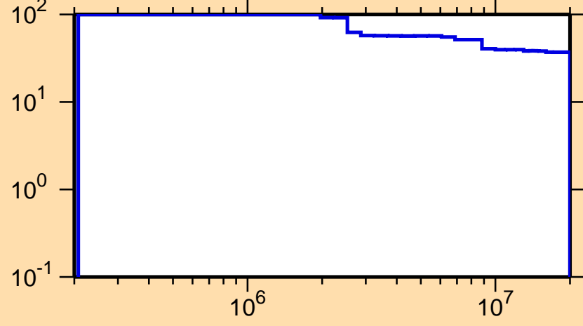
\Delta\sigma/\sigma vs. E for ^{119}\text{La}(n,n\text{cont.})
