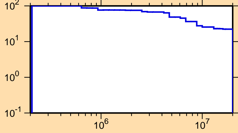
\Delta\sigma/\sigma vs. E for ^{119}\text{La}(n,n_1)
