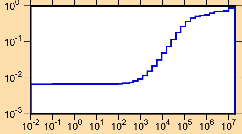
\mu vs. E for ^{119}\text{La}(\text{mt251})
