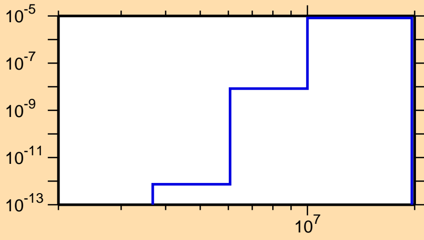
\sigma vs. E for ^{119}\text{La}(\text{mt117})
