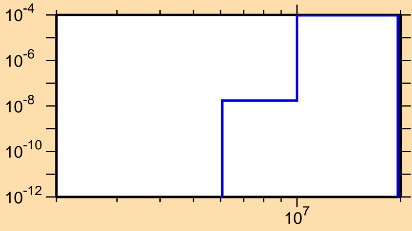
\sigma vs. E for ^{119}\text{La} (mt 45)
