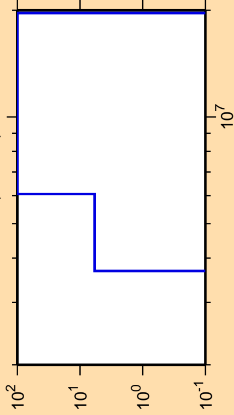
\Delta\sigma/\sigma vs. E for ^{119}\text{La}(\text{mt117})
