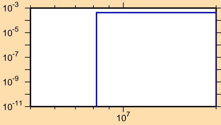
\sigma vs. E for ^{119}\text{La}(n,t)
