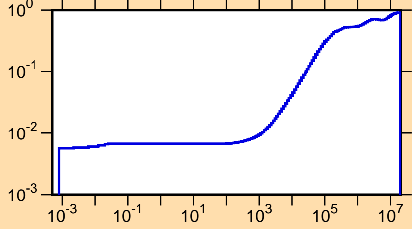
\mu vs. E for ^{120}\text{La}(\text{mt251})
