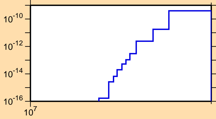
\sigma vs. E for ^{120}\text{La}(n,2n\alpha)
