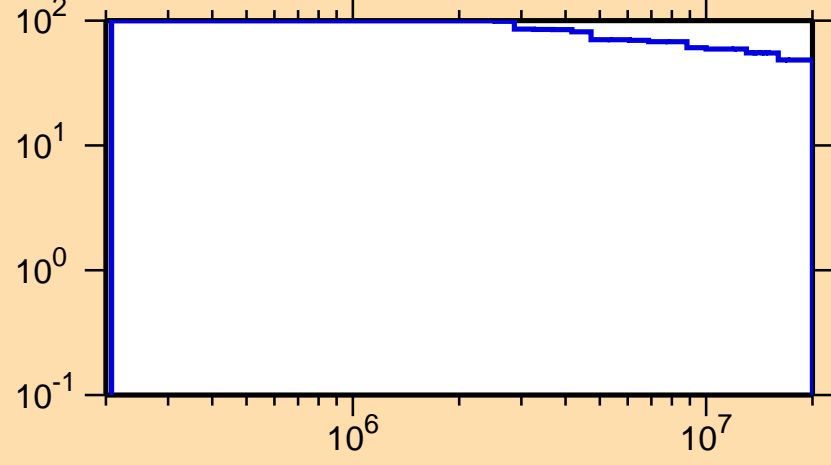
\Delta\sigma/\sigma vs. E for ^{120}\text{La}(n,n\text{cont.})
