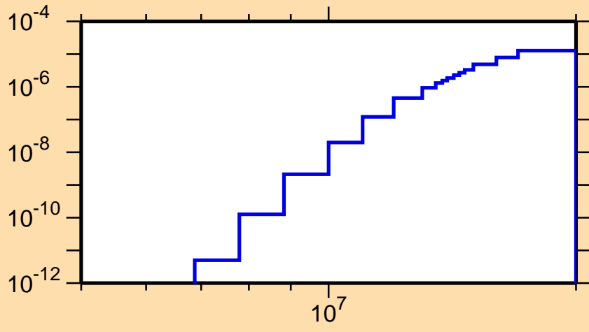
\sigma vs. E for ^{120}\text{La}(\text{mt117})
