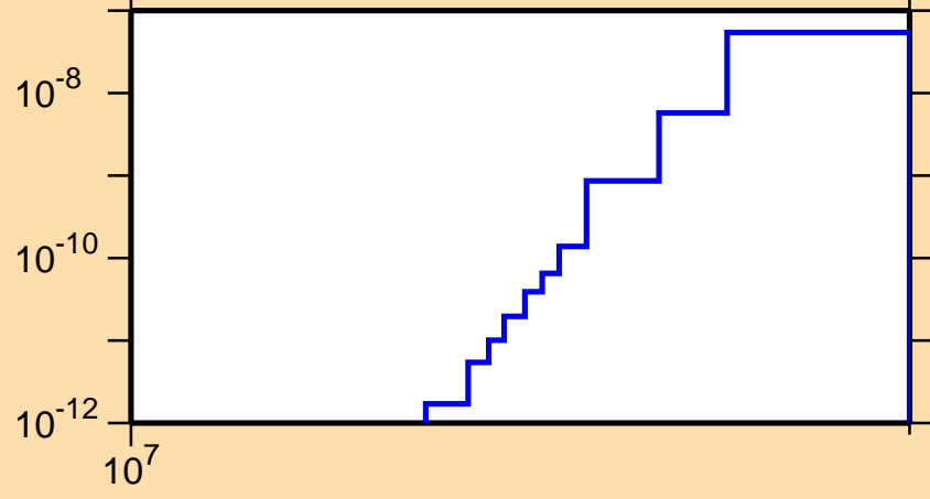
\sigma vs. E for ^{120}\text{La} (mt 34)
