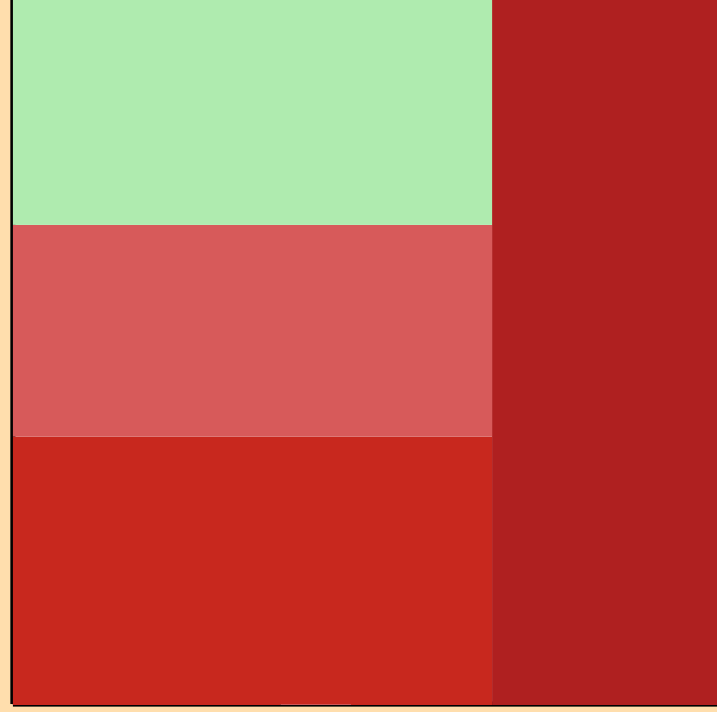
\Delta\sigma/\sigma vs. E for ^{120}\text{La}(n,2n)
