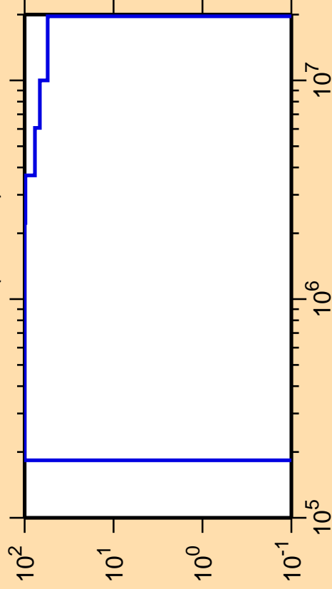
\Delta\sigma/\sigma vs. E for ^{120}\text{La}(n,\text{inel.})
