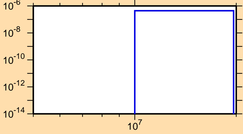
\sigma vs. E for ^{120}\text{La}(n,\text{nd})
