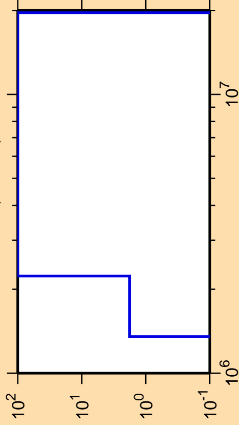
\Delta\sigma/\sigma vs. E for ^{120}\text{La}(n,\text{He3})
