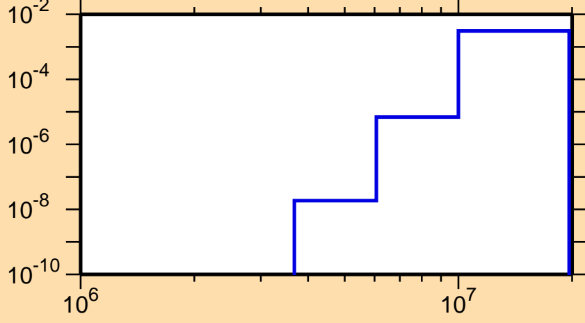
\sigma vs. E for ^{120}\text{La}(n,\text{He3})
