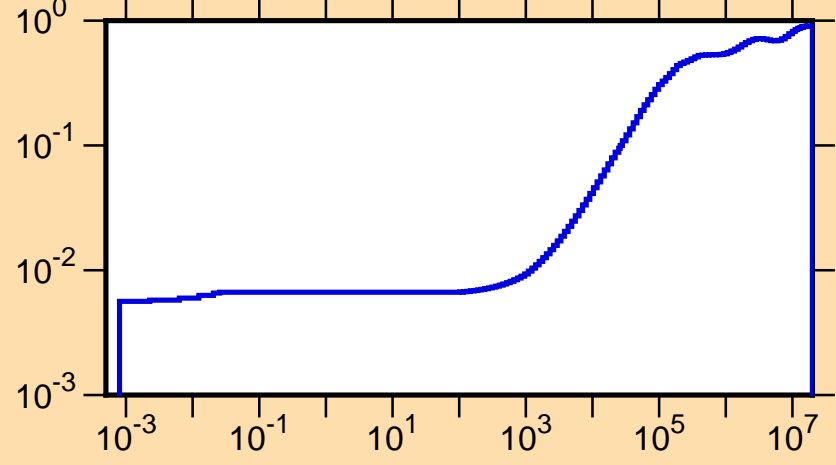
\mu vs. E for ^{121}\text{La}(\text{mt251})
