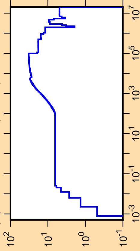
\Delta\mu/\mu vs. E for ^{121}\text{La}(\text{mt251})
