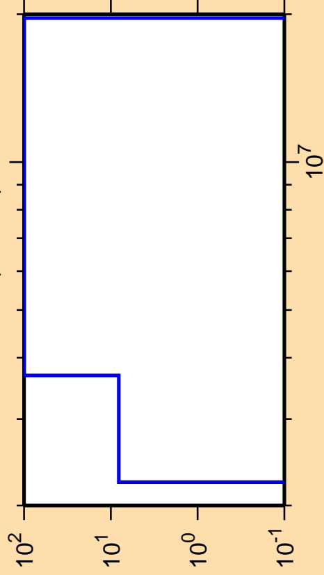
\Delta\sigma/\sigma vs. E for ^{121}\text{La}(n,\text{He3})
