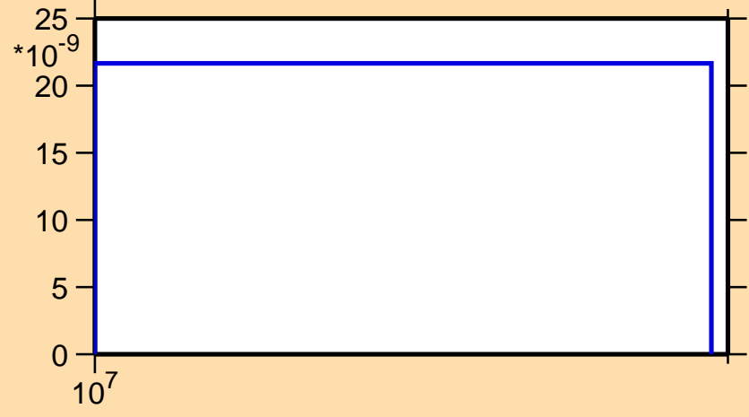
\sigma vs. E for ^{121}\text{La}(n,\text{nd})
