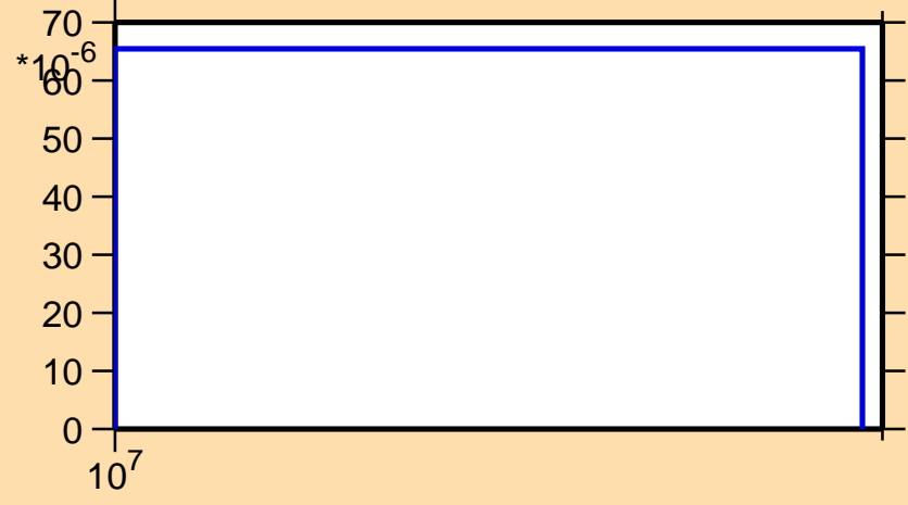
\sigma vs. E for ^{121}\text{La}(n,2n)
