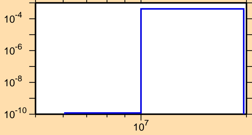
\sigma vs. E for ^{121}\text{La}(n,t)
