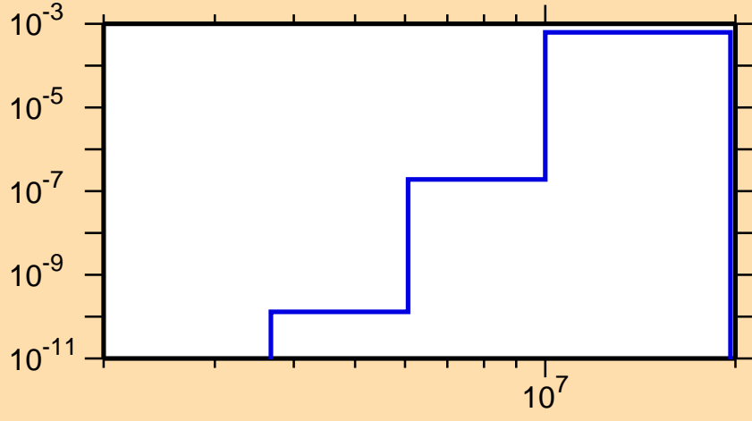
\sigma vs. E for ^{121}\text{La}(n,\text{He3})
