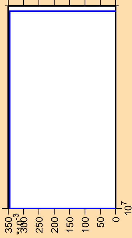
\Delta\sigma/\sigma vs. E for ^{121}\text{La}(n,2n\alpha)
