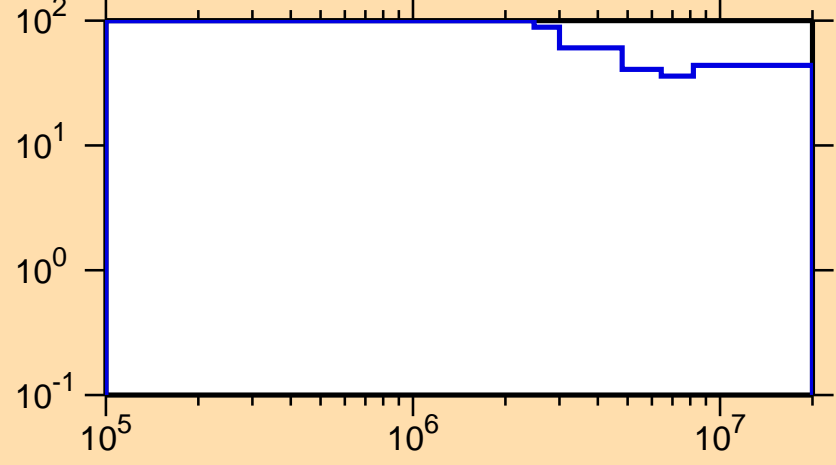
\Delta\sigma/\sigma vs. E for ^{121}\text{La}(n,n_{cont.})
