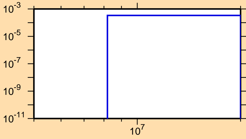
\sigma vs. E for ^{121}\text{La}(n,t)
