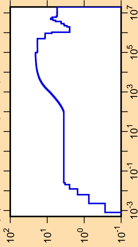
\Delta\mu/\mu vs. E for ^{122}\text{La}(\text{mt251})
