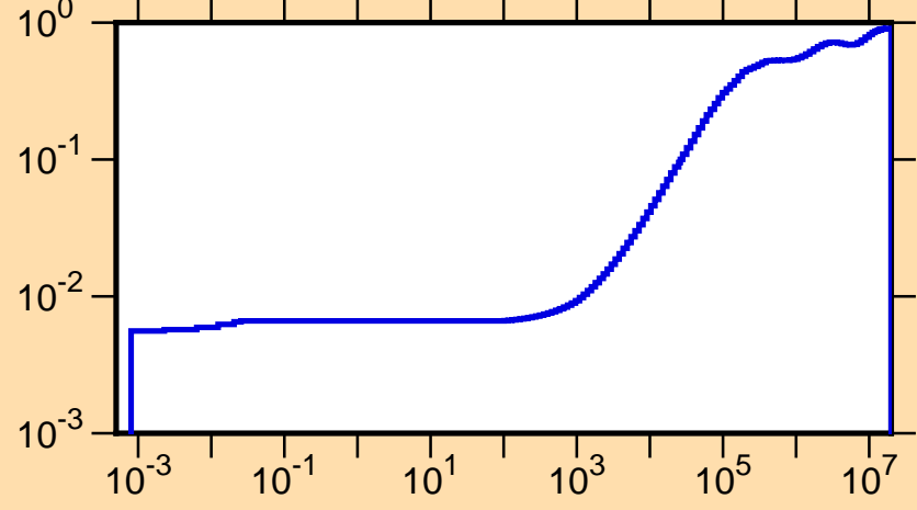
\mu vs. E for ^{122}\text{La}(\text{mt251})
