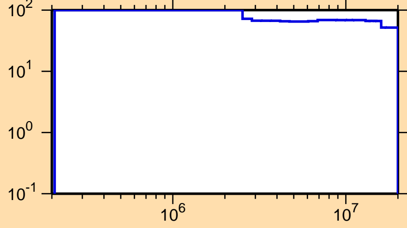
\Delta\sigma/\sigma vs. E for ^{122}\text{La}(n,n\text{cont.})
