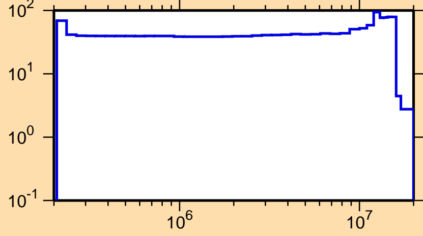
\Delta\sigma/\sigma vs. E for ^{122}\text{La}(n,n_1)
