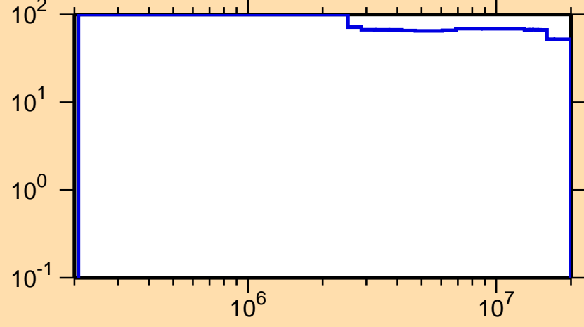
\Delta\sigma/\sigma vs. E for ^{122}\text{La}(n,\text{inel.})
