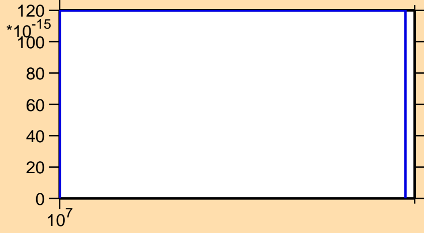
\sigma vs. E for ^{122}\text{La}(n,nt)
