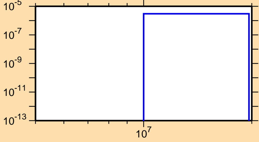
\sigma vs. E for ^{122}\text{La}(n,\text{nd})
