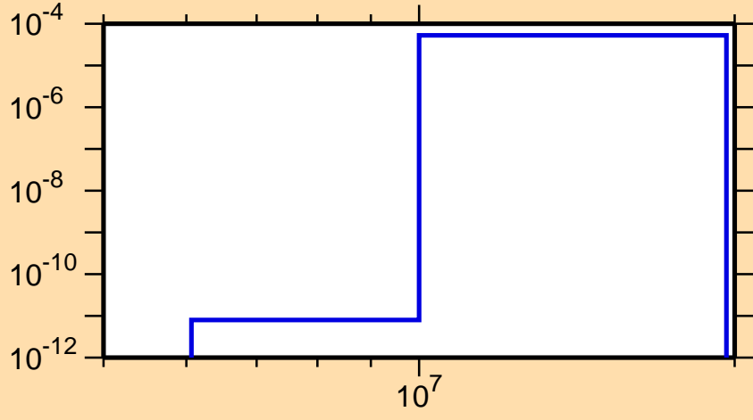
\sigma vs. E for ^{122}\text{La} (mt 45)
