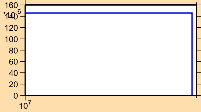
\sigma vs. E for ^{122}\text{La}(n,2np)
