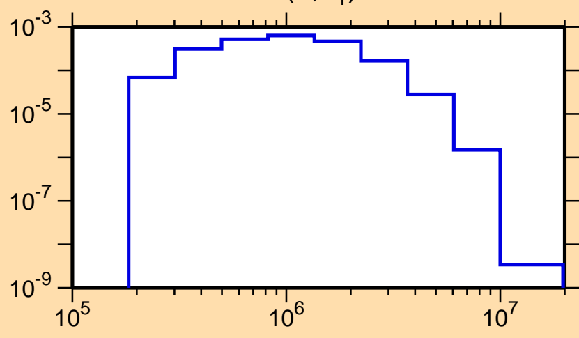
\sigma vs. E for ^{122}\text{La}(n,n_1)
