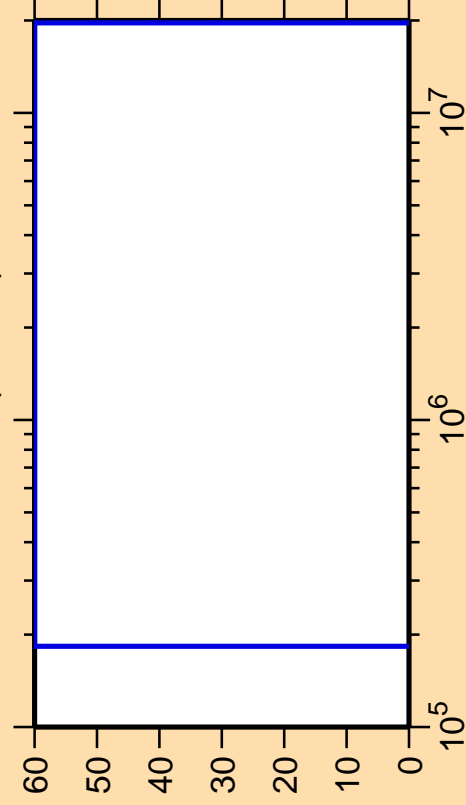
\Delta\sigma/\sigma vs. E for ^{122}\text{La}(n,\text{inel.})
