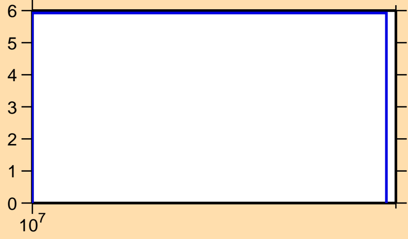
\Delta\sigma/\sigma vs. E for ^{122}\text{La}(n,\text{el.})
