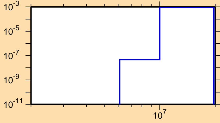
\sigma vs. E for ^{122}\text{La}(n,t)
