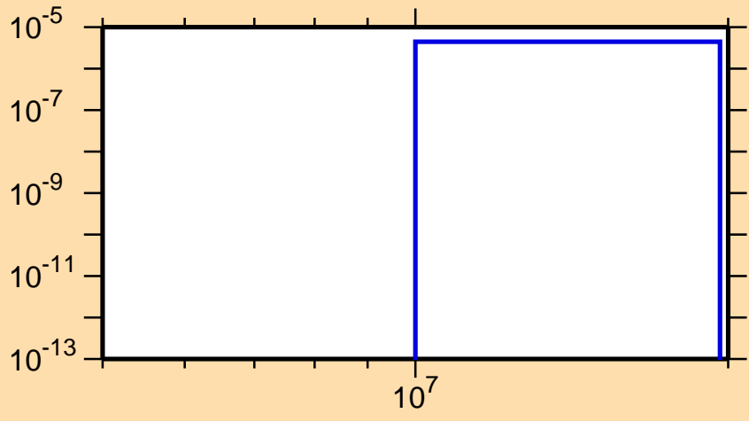
\sigma vs. E for ^{122}\text{La}(n,\text{pt})
