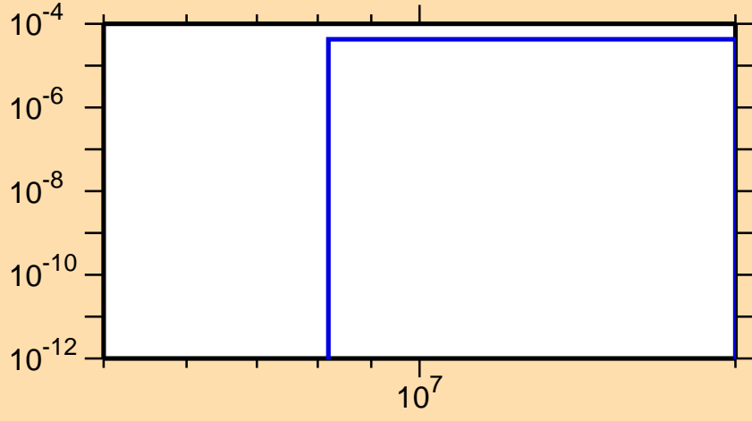
\sigma vs. E for ^{122}\text{La} (mt 45)
