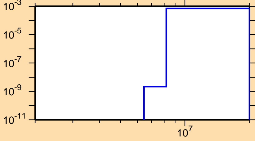
\sigma vs. E for ^{122}\text{La}(n,t)
