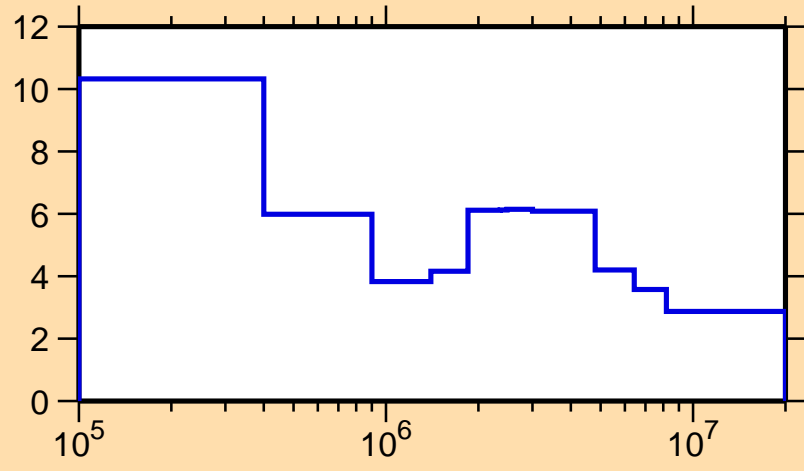
\Delta\sigma/\sigma vs. E for ^{122}\text{La}(n,\text{tot.})
