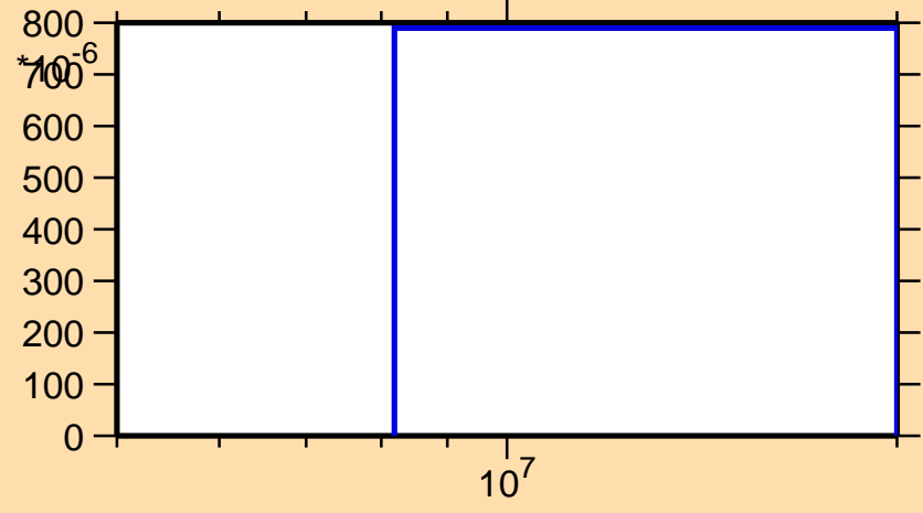
\sigma vs. E for ^{122}\text{La}(n,2n)
