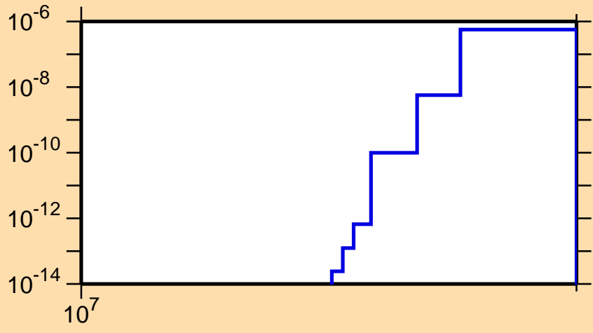
\sigma vs. E for ^{123}\text{La}(n,pt)
