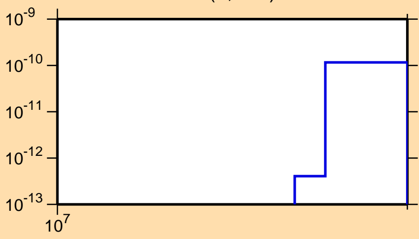
\sigma vs. E for ^{123}\text{La}(n,2n\alpha)
