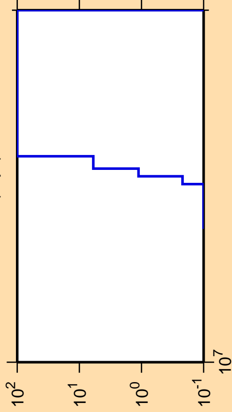
\Delta\sigma/\sigma vs. E for ^{123}\text{La}(n,pt)
