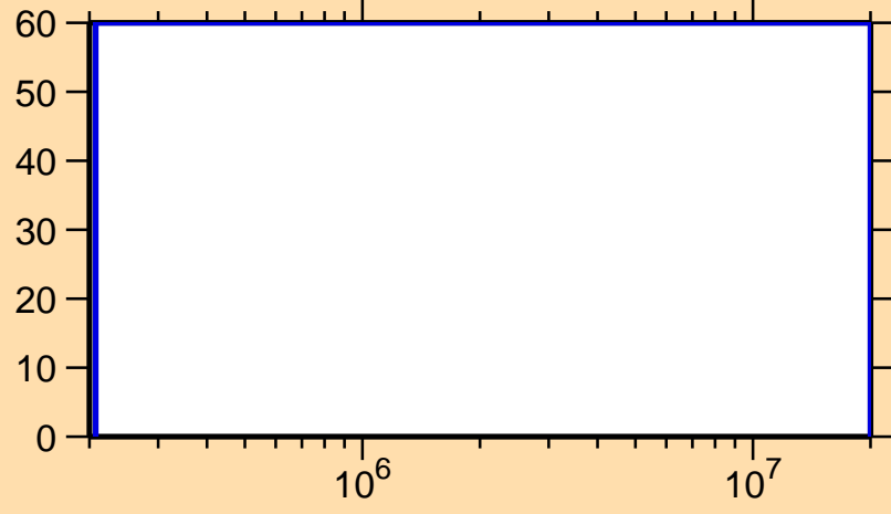
\Delta\sigma/\sigma vs. E for ^{123}\text{La}(n,n\text{cont.})
