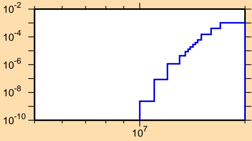
\sigma vs. E for ^{123}\text{La}(n,pd)
