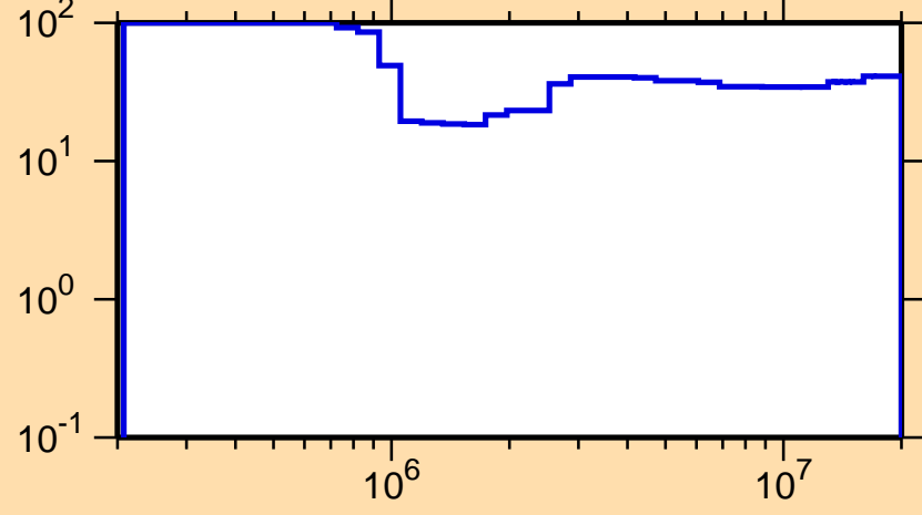
\Delta\sigma/\sigma vs. E for ^{123}\text{La}(n,n_1)
