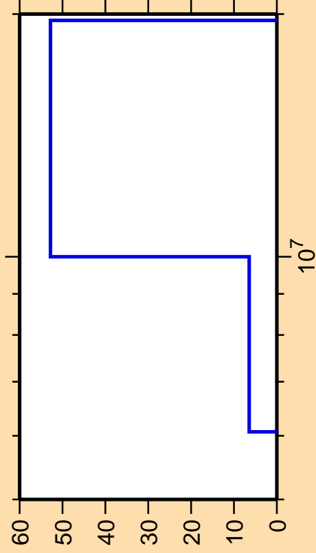
\Delta\sigma/\sigma vs. E for ^{123}\text{La}(\text{mt } 45)
