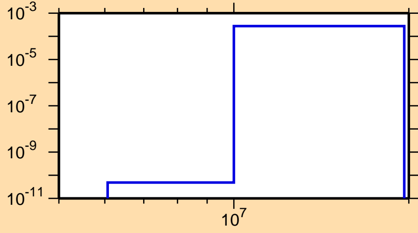
\sigma vs. E for ^{123}\text{La}(n,t)
