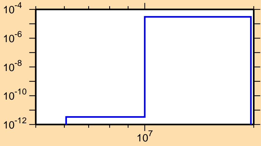
\sigma vs. E for ^{123}\text{La}(\text{mt } 45)
