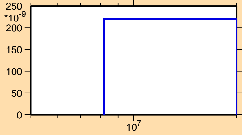
\sigma vs. E for ^{123}\text{La}(\text{mt117})
