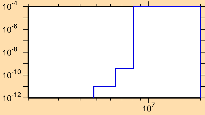
\sigma vs. E for ^{123}\text{La}(n,\text{He3})
