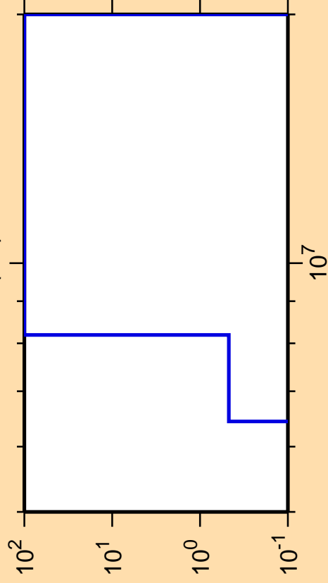
\Delta\sigma/\sigma vs. E for ^{123}\text{La}(n,t)
