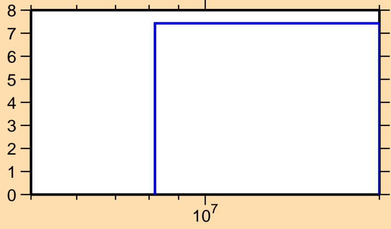
\Delta\sigma/\sigma vs. E for ^{123}\text{La}(n,\text{el.})
