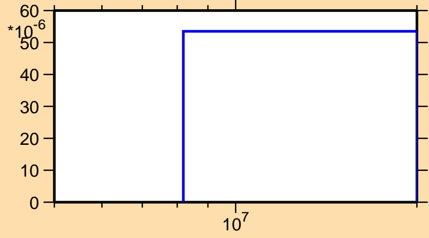
\sigma vs. E for ^{123}\text{La}(n,\text{pd})
