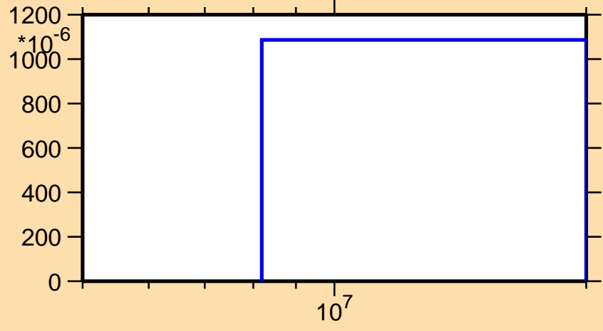
\sigma vs. E for ^{123}\text{La}(n,2n)
