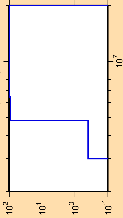
\Delta\sigma/\sigma vs. E for ^{123}\text{La}(n,\text{He3})
