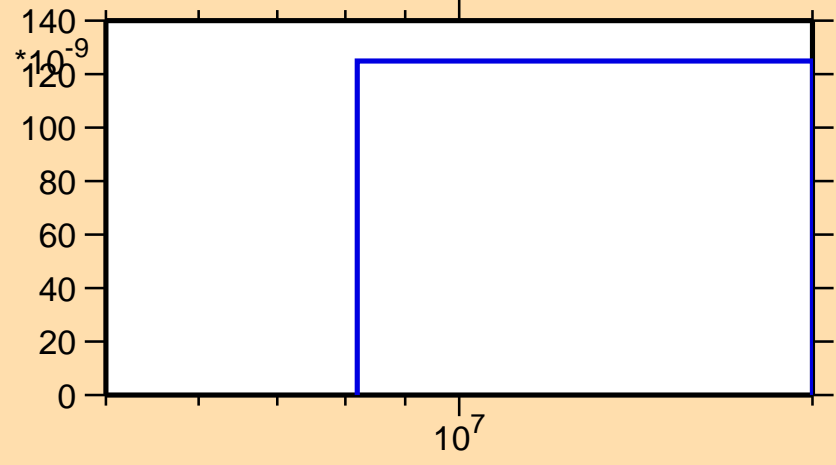
\sigma vs. E for ^{123}\text{La}(n,\text{nd})
