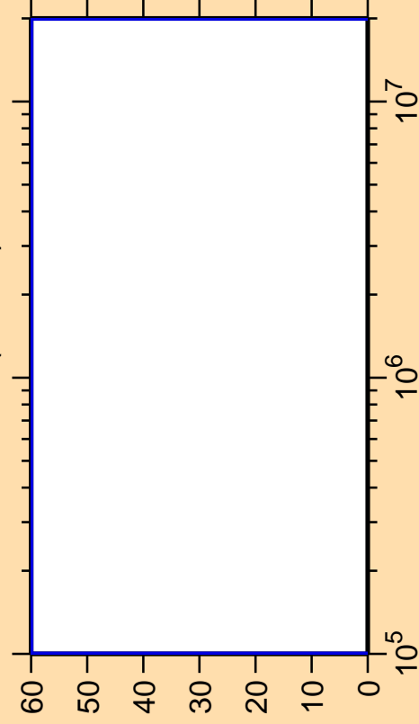
\Delta\sigma/\sigma vs. E for ^{123}\text{La}(n,\text{inel.})
