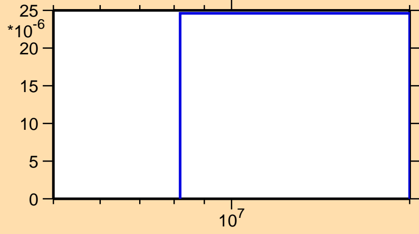
\sigma vs. E for ^{123}\text{La} (mt 45)
