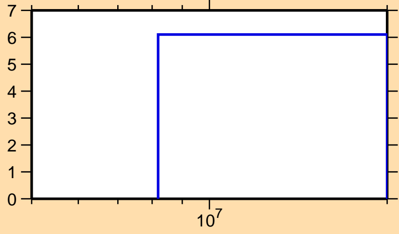
\Delta\sigma/\sigma vs. E for ^{123}\text{La}(n,\text{tot.})
