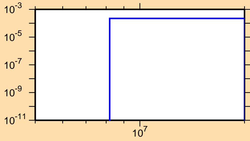
\sigma vs. E for ^{123}\text{La}(n,t)
