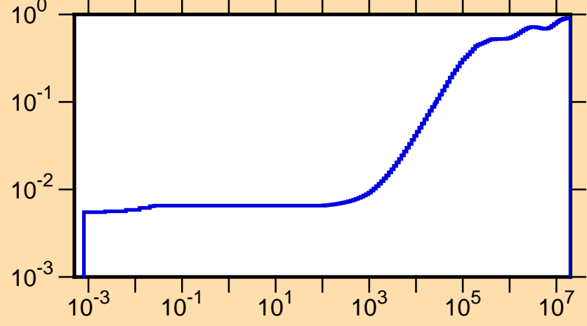
\mu vs. E for ^{124}\text{La}(\text{mt251})
