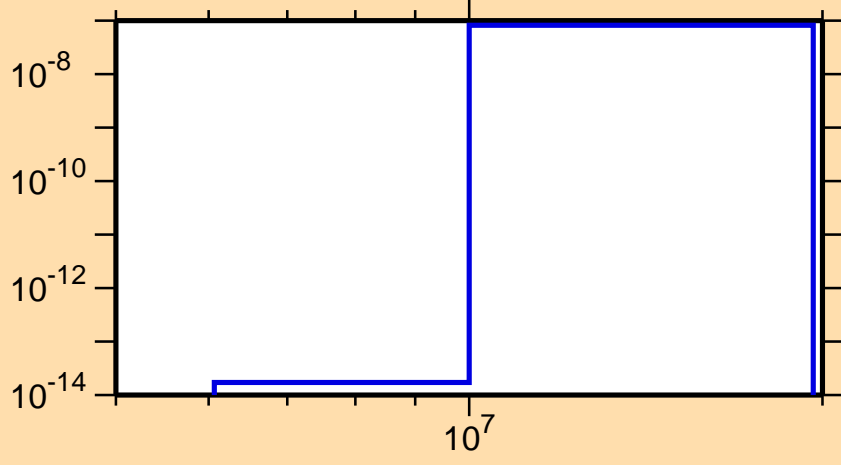
\sigma vs. E for ^{124}\text{La}(\text{mt117})
