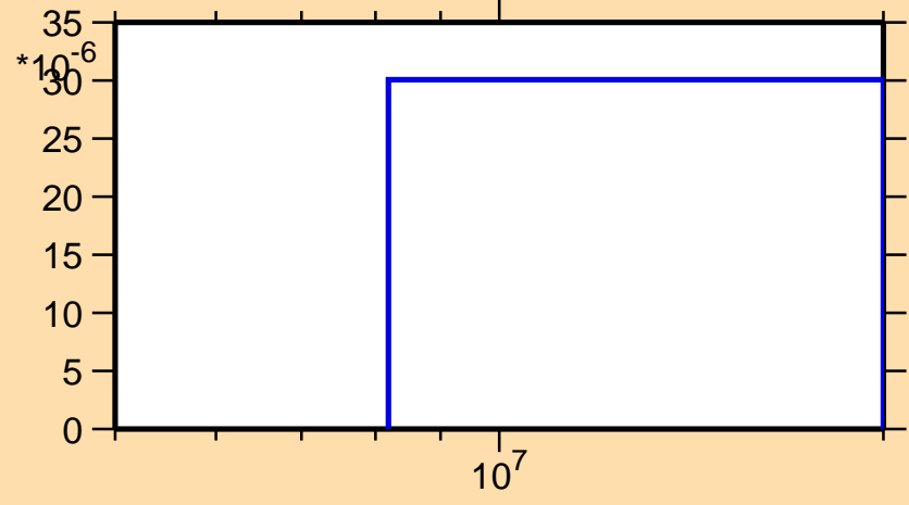
\sigma vs. E for ^{124}\text{La}(n,pd)
