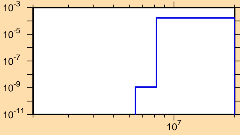
\sigma vs. E for ^{124}\text{La}(n,\text{He}3)
