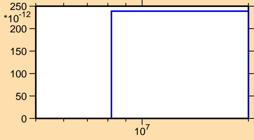
\sigma vs. E for ^{124}\text{La}(\text{mt } 34)
