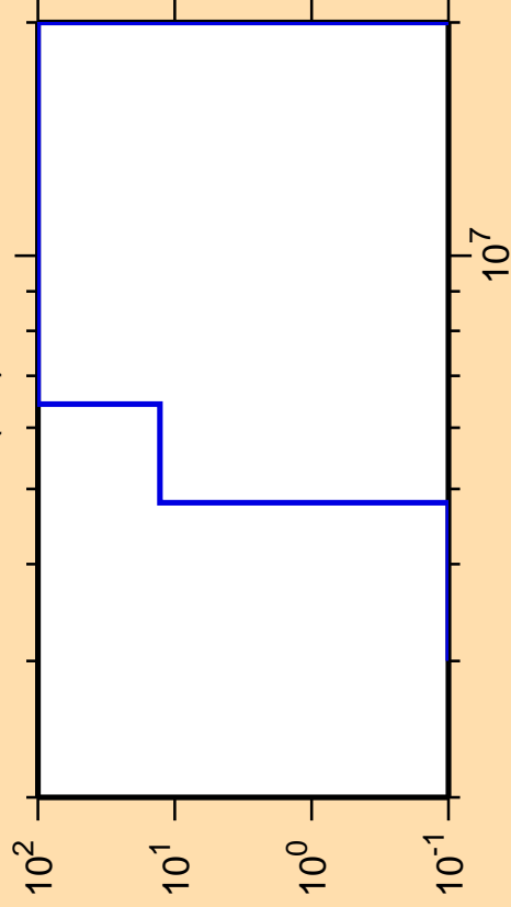
\Delta\sigma/\sigma vs. E for ^{124}\text{La}(n,t)
