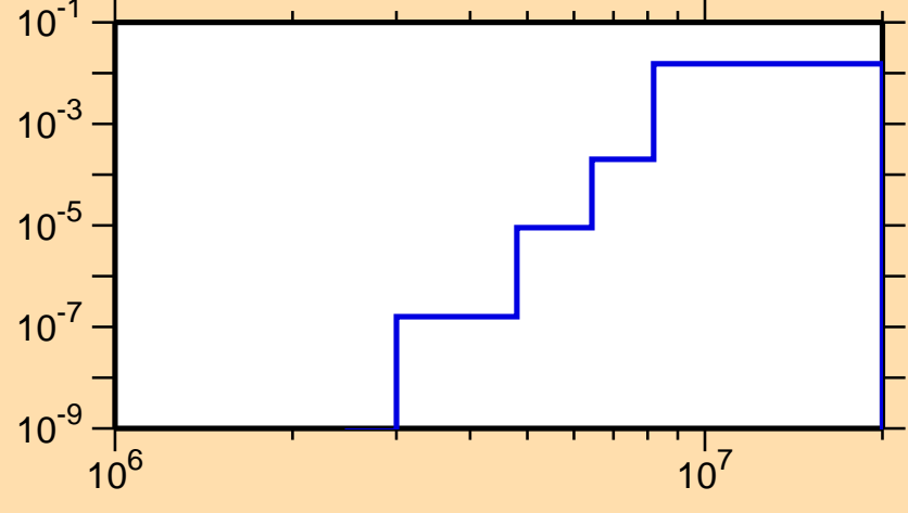
\sigma vs. E for ^{124}\text{La}(n,d)
