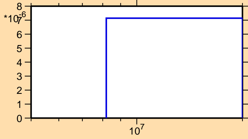
\sigma vs. E for ^{124}\text{La}(\text{mt } 45)
