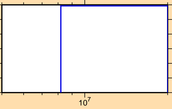
\sigma vs. E for ^{124}\text{La}(n,2np)
