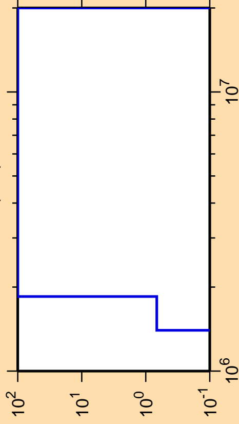
\Delta\sigma/\sigma vs. E for ^{124}\text{La}(n,d)
