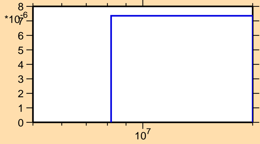
\sigma vs. E for ^{124}\text{La}(n,\text{nd})
