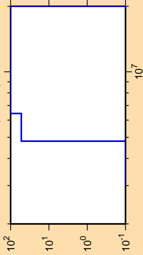
\Delta\sigma/\sigma vs. E for ^{124}\text{La}(n,\text{He}3)
