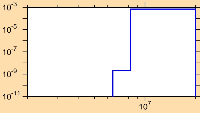
\sigma vs. E for ^{124}\text{La}(n,t)
