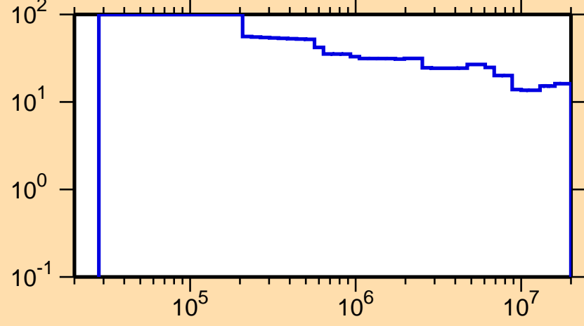
\Delta\sigma/\sigma vs. E for ^{124}\text{La}(n,\text{tot.})
