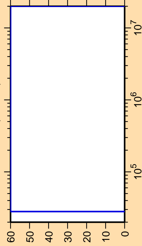
\Delta\sigma/\sigma vs. E for ^{124}\text{La}(n,\text{inel.})
