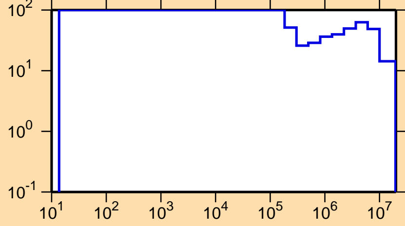
\Delta\sigma/\sigma vs. E for ^{124}\text{La}(n,\text{el.})
