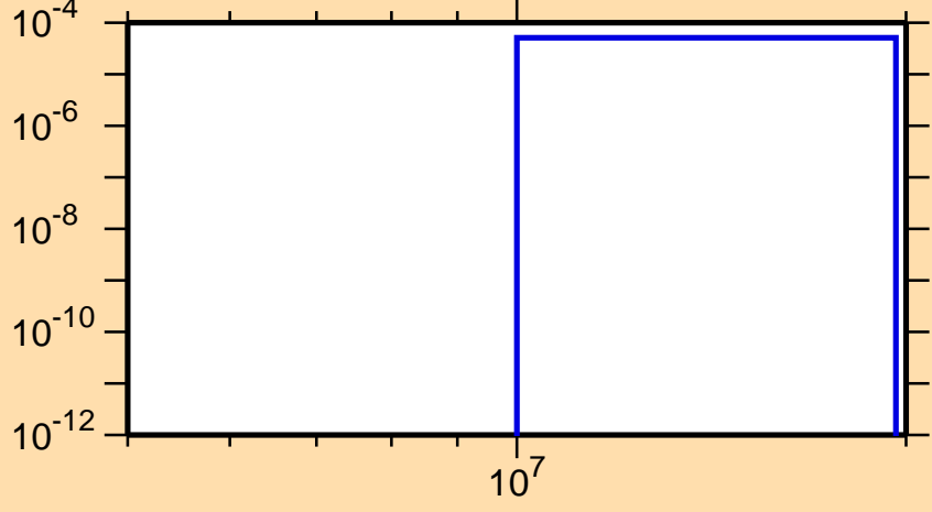
\sigma vs. E for ^{124}\text{La}(n,nd)
