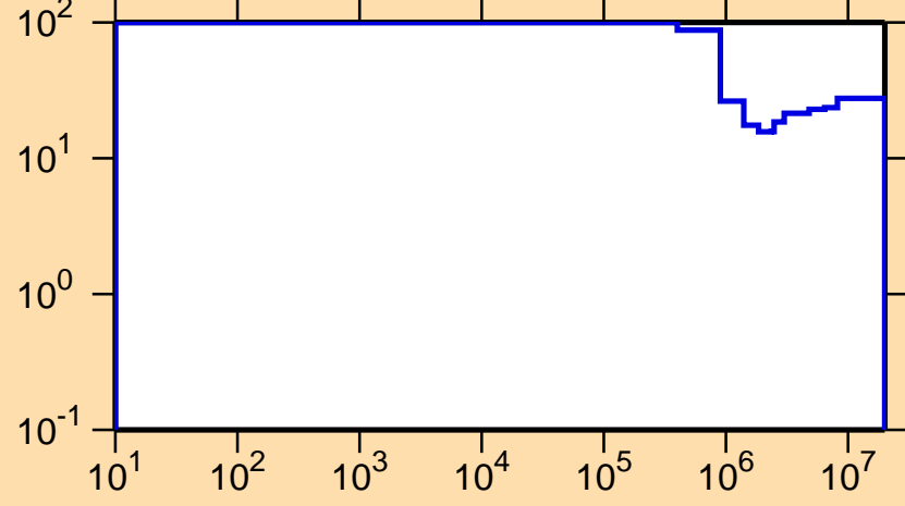
\Delta\sigma/\sigma vs. E for ^{124}\text{La}(n,\text{nonel.})
