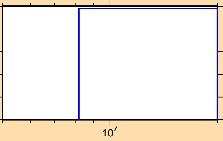
\sigma vs. E for ^{124}\text{La}(n,2n\alpha)
