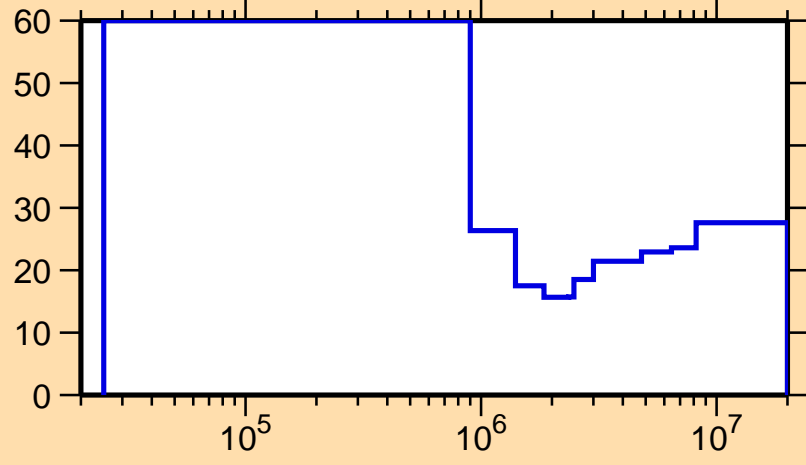
\Delta\sigma/\sigma vs. E for ^{124}\text{La}(n,n\text{onel.})
