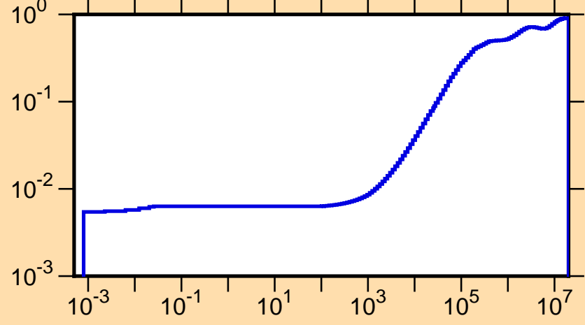
\mu vs. E for ^{125}\text{La}(\text{mt251})
