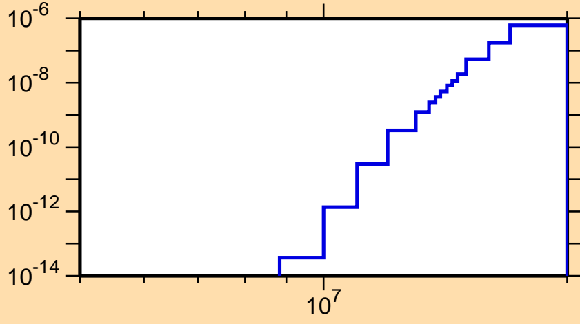
\sigma vs. E for ^{125}\text{La}(\text{mt117})
