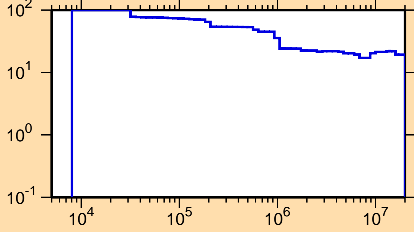
\Delta\sigma/\sigma vs. E for ^{125}\text{La}(n,\text{nonel.})
