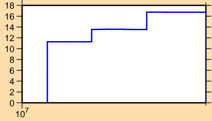
\Delta\sigma/\sigma vs. E for ^{125}\text{La}(n,\text{el.})
