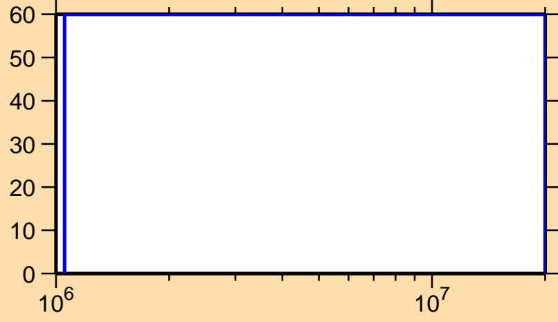
\Delta\sigma/\sigma vs. E for ^{125}\text{La}(n,n_1)
