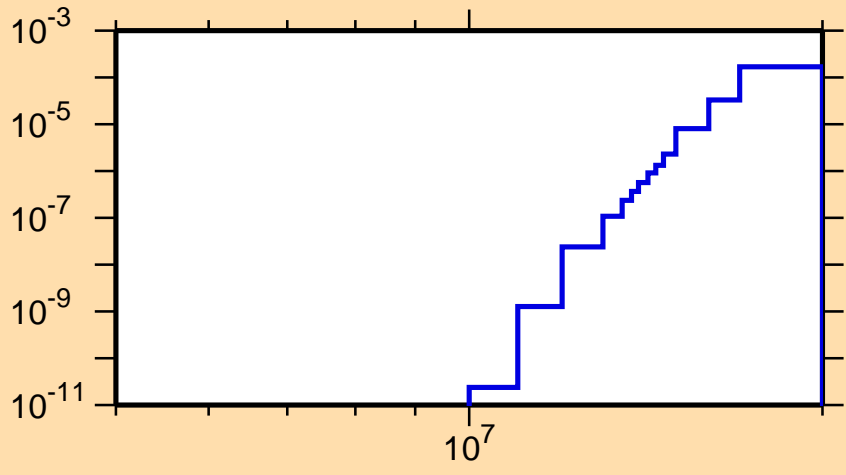
\sigma vs. E for ^{125}\text{La} (mt 45)
