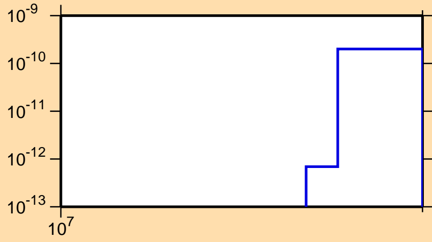
\sigma vs. E for ^{125}\text{La} (mt 34)
