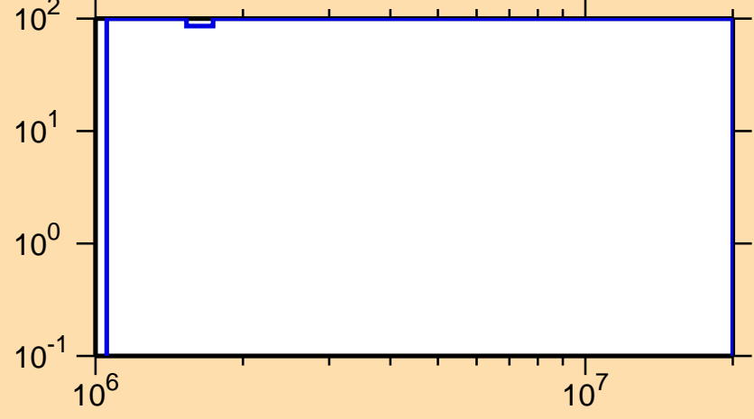
\Delta\sigma/\sigma vs. E for ^{125}\text{La}(n,ncont.)
