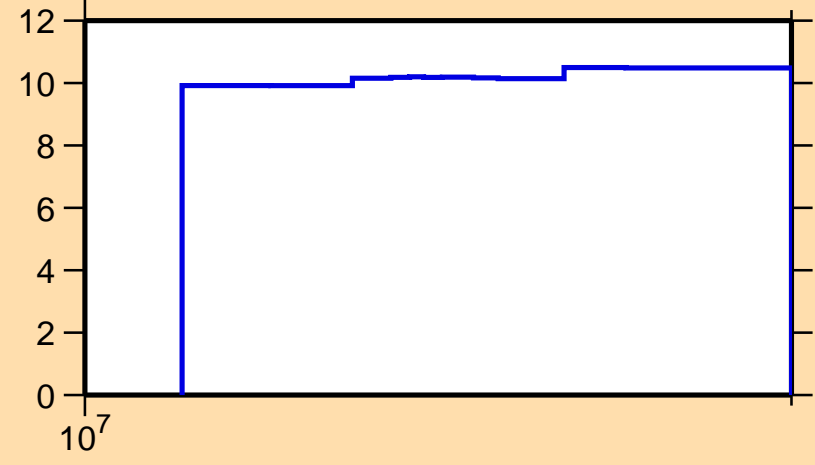
\Delta\sigma/\sigma vs. E for ^{125}\text{La}(n,\text{tot.})
