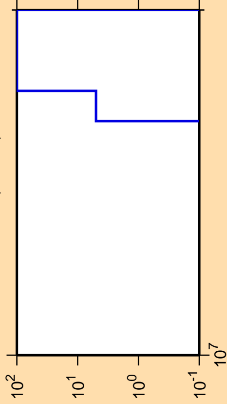
\Delta\sigma/\sigma vs. E for ^{125}\text{La} (mt 34)
