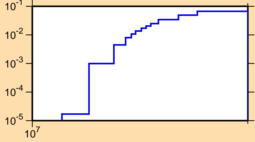
\sigma vs. E for ^{125}\text{La}(n,2n)
