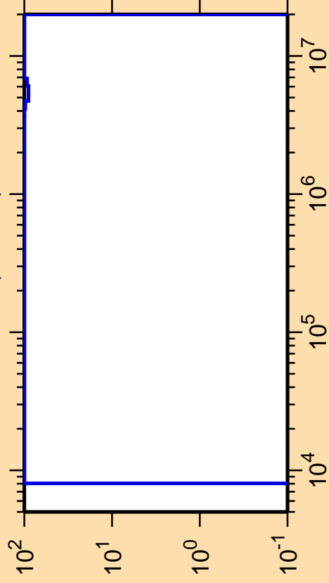
\Delta\sigma/\sigma vs. E for ^{125}\text{La}(n,\text{inel.})
