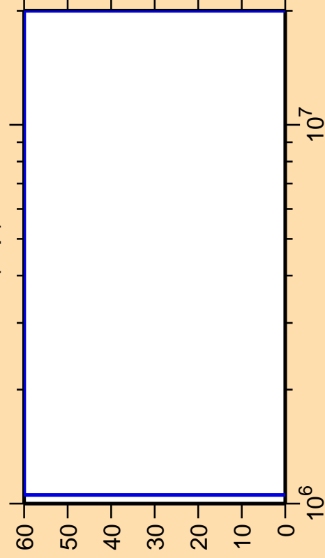
\Delta\sigma/\sigma vs. E for ^{125}\text{La}(n,p)
