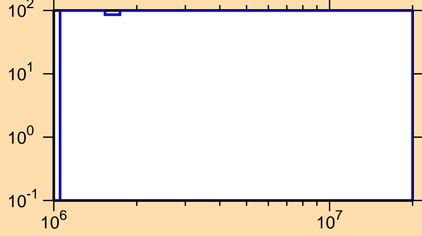
\Delta\sigma/\sigma vs. E for ^{125}\text{La}(n,n\text{cont.})
