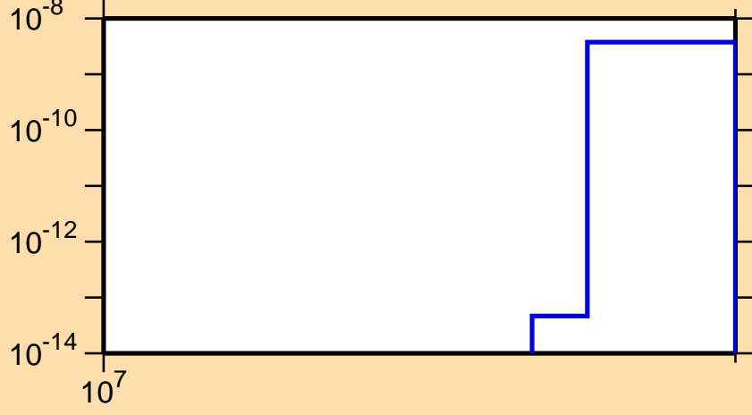
\sigma vs. E for ^{125}\text{La}(n,nt)
