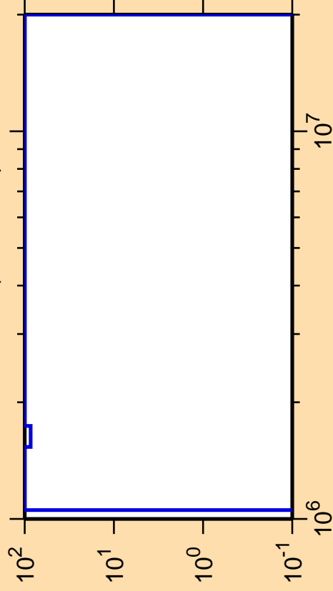
\Delta\sigma/\sigma vs. E for ^{125}\text{La}(n,n_{\text{cont}}) .
