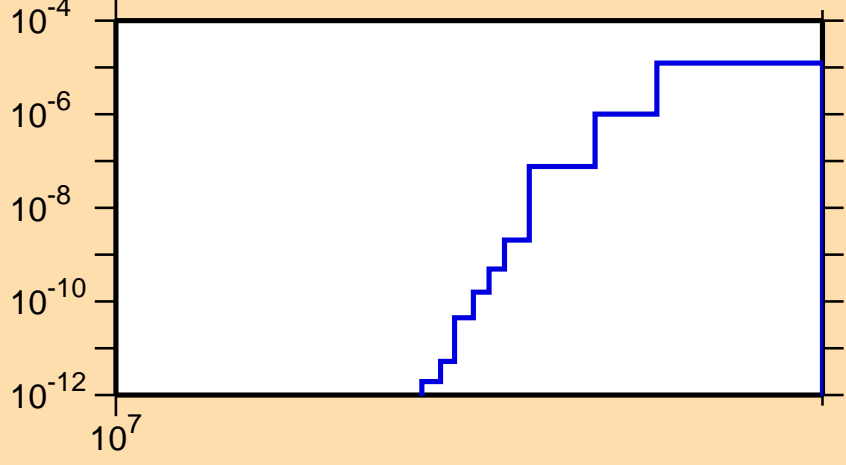
\sigma vs. E for ^{125}\text{La}(n,\text{nd})
