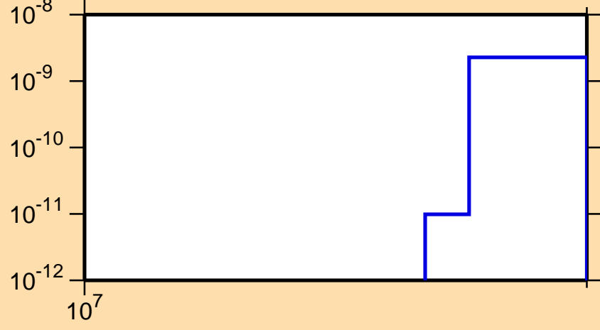
\sigma vs. E for ^{125}\text{La}(n,2n\alpha)
