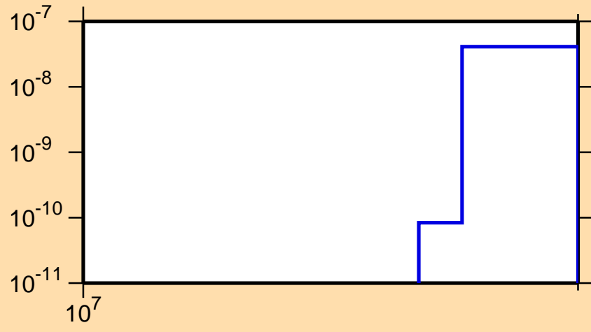
\sigma vs. E for ^{125}\text{La}(n,\text{pt})
