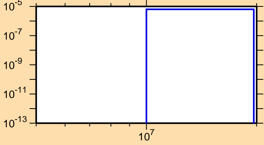
\sigma vs. E for ^{125}\text{La}(n,pd)
