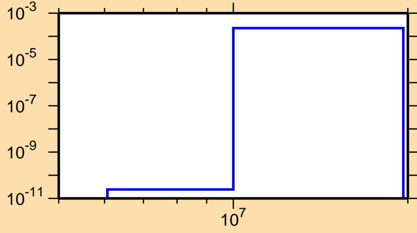
\sigma vs. E for ^{125}\text{La}(n,t)
