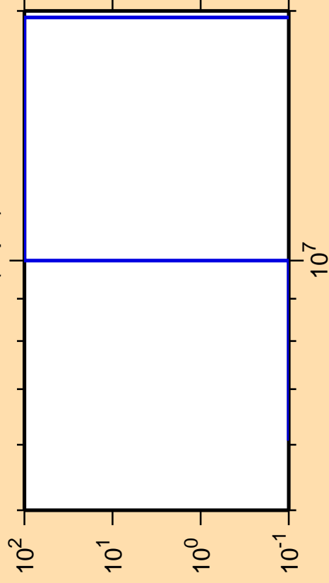
\Delta\sigma/\sigma vs. E for ^{125}\text{La}(n,pd)
