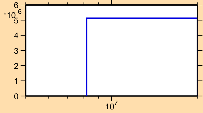
\sigma vs. E for ^{125}\text{La}(n,\text{pd})
