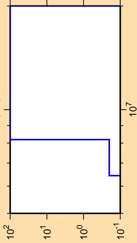
\Delta\sigma/\sigma vs. E for ^{125}\text{La}(n,t)
