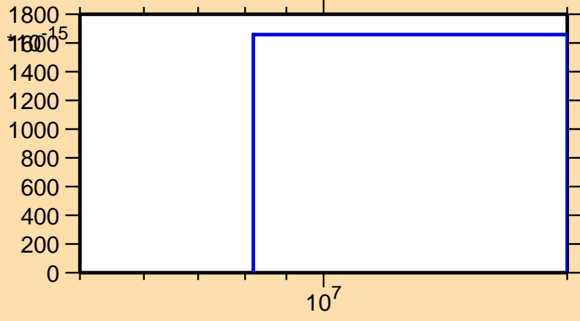
\sigma vs. E for ^{125}\text{La} (mt 34)
