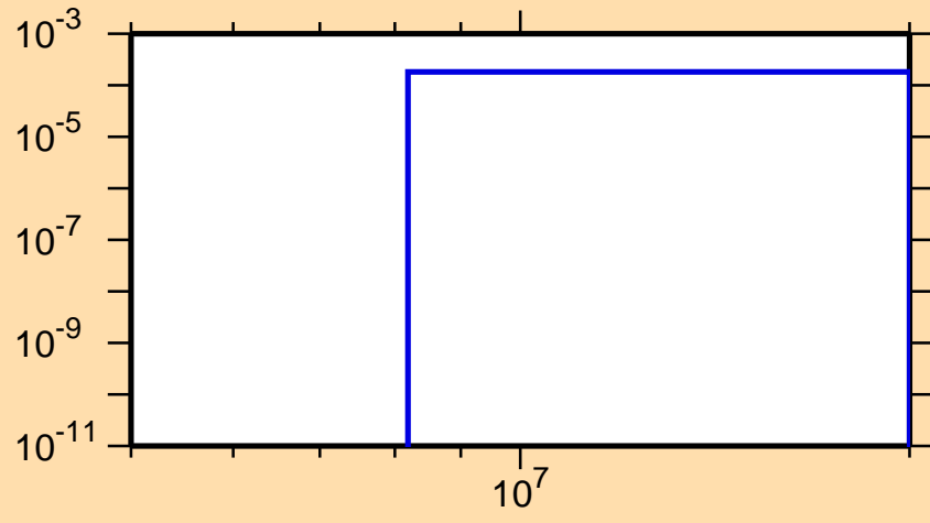
\sigma vs. E for ^{125}\text{La}(n,t)
