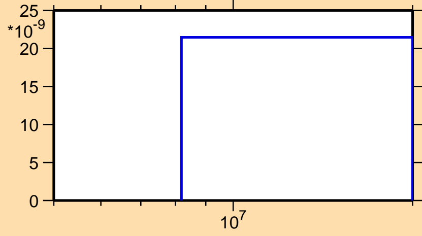
\sigma vs. E for ^{125}\text{La}(\text{mt117})
