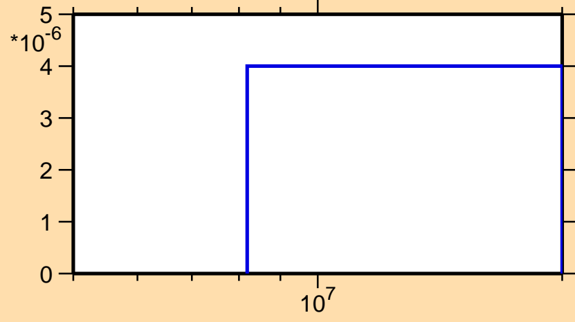
\sigma vs. E for ^{125}\text{La} (mt 45)
