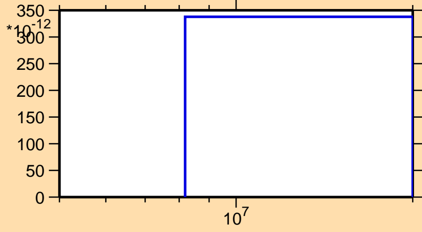
\sigma vs. E for ^{125}\text{La}(n,\text{pt})
