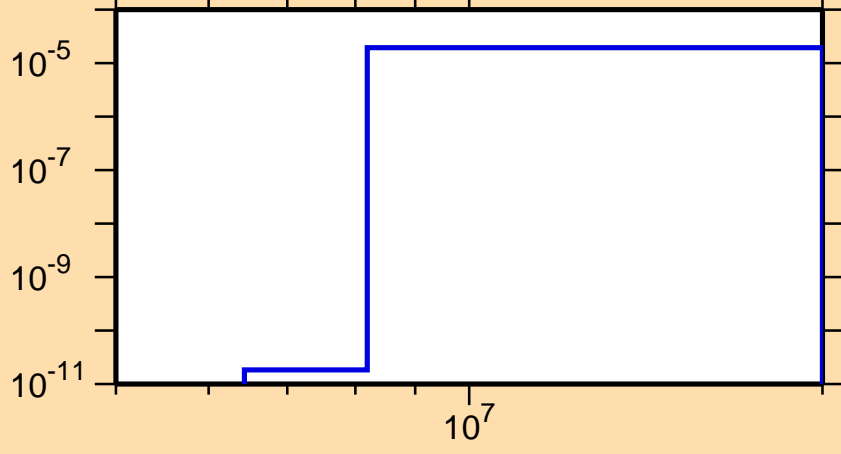
\sigma vs. E for ^{125}\text{La}(n,\text{He3})
