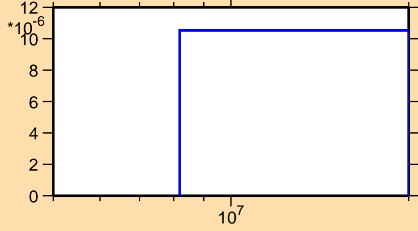
\sigma vs. E for ^{125}\text{La}(n,2np)
