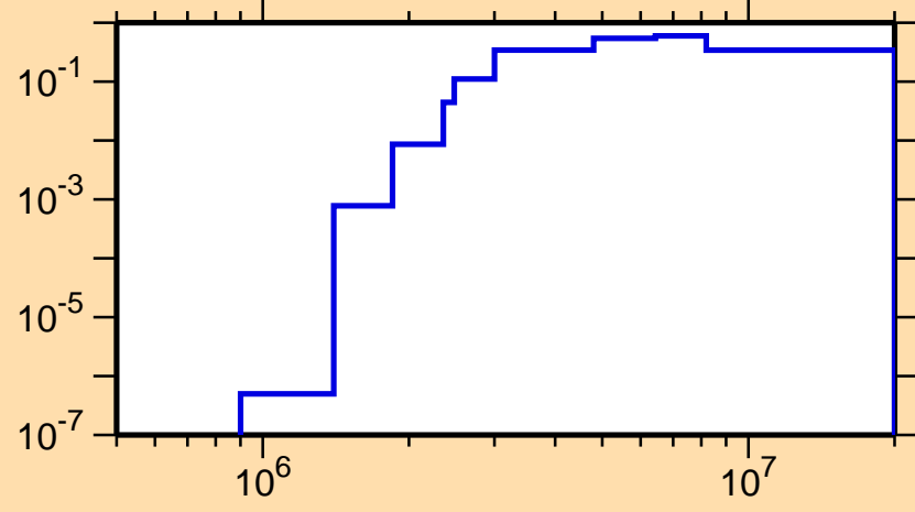
\sigma vs. E for ^{125}\text{La}(n,n\text{cont.})
